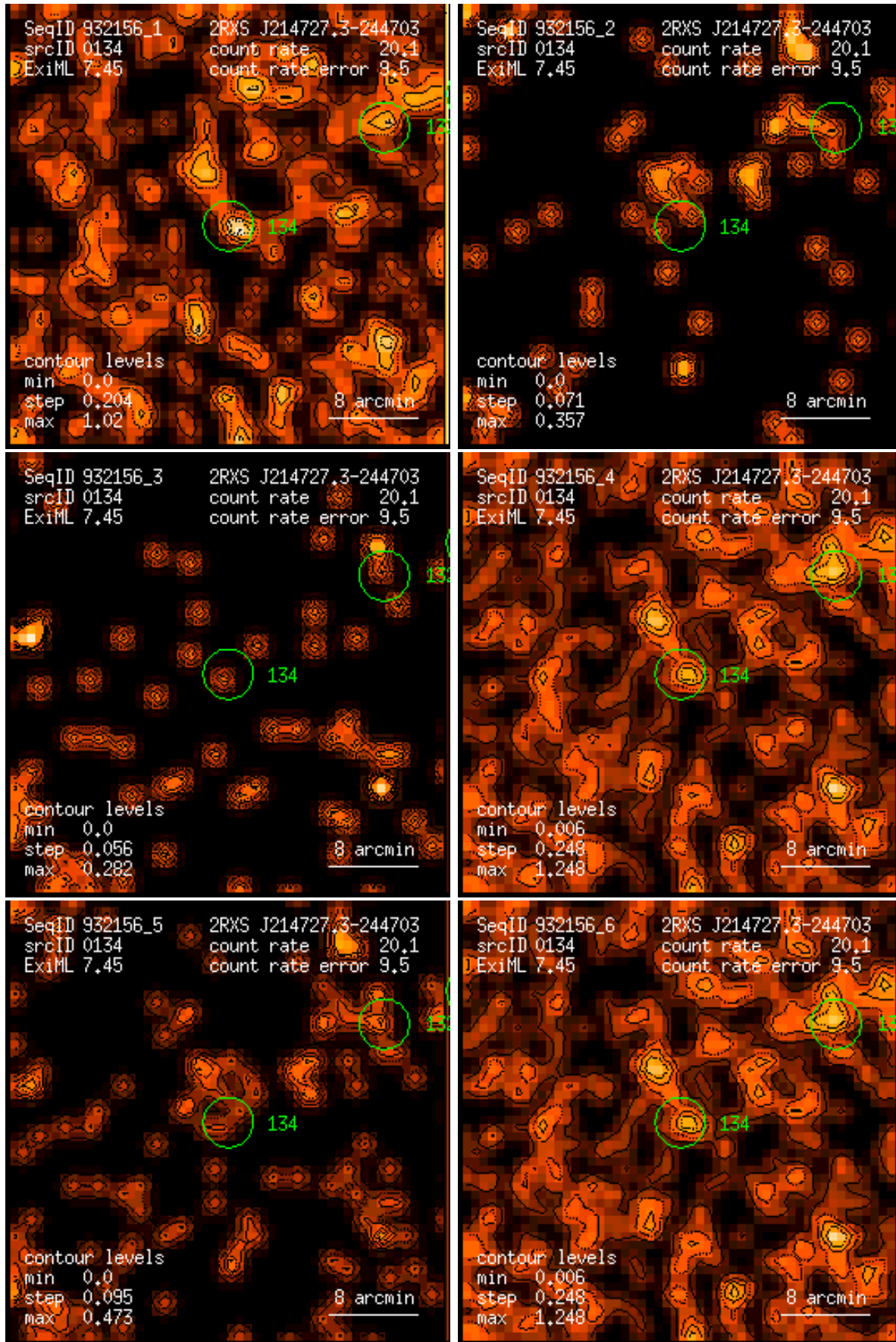
Figure 134: RASS 932156: detection 0134: band rate images, Gaussian filter: (1) PSPC channels 11 – 41, (2) 52 – 90, (3) 91 – 201, (4) 11 – 235, (5) 52 – 201, (6) 11 – 201. Broad band rates in counts/ks. Band rate contour levels in counts/ks/arcmin 2 .
