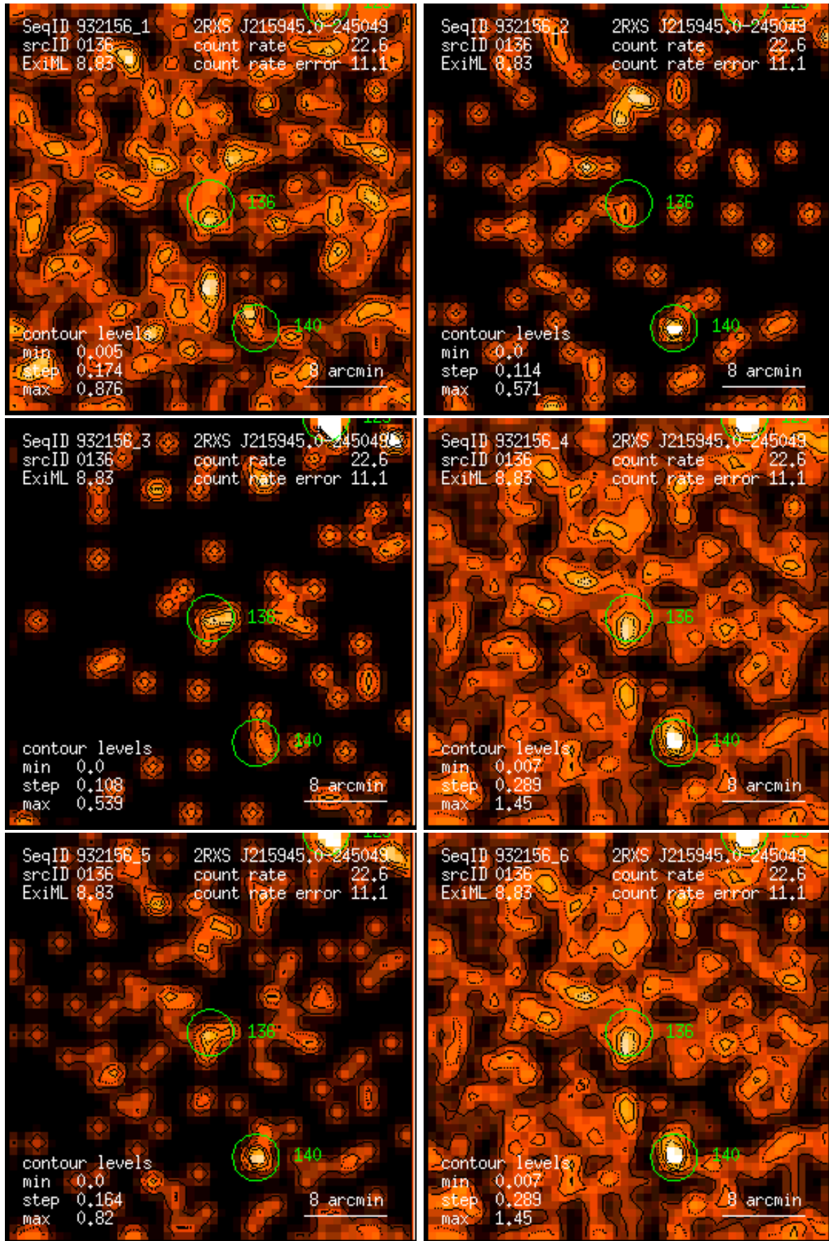
Figure 136: RASS 932156: detection 0136: band rate images, Gaussian filter: (1) PSPC channels 11 – 41, (2) 52 – 90, (3) 91 – 201, (4) 11 – 235, (5) 52 – 201, (6) 11 – 201. Broad band rates in counts/ks. Band rate contour levels in counts/ks/arcmin 2 .
