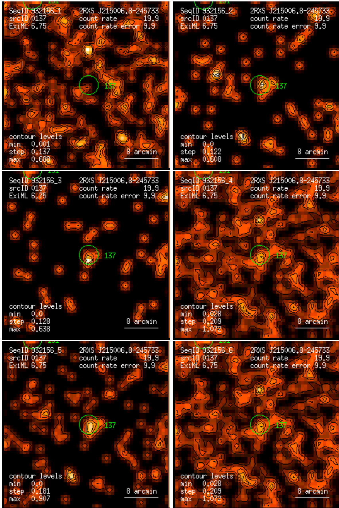
Figure 137: RASS 932156: detection 0137: band rate images, Gaussian filter: (1) PSPC channels 11 – 41, (2) 52 – 90, (3) 91 – 201, (4) 11 – 235, (5) 52 – 201, (6) 11 – 201. Broad band rates in counts/ks. Band rate contour levels in counts/ks/arcmin 2 .
