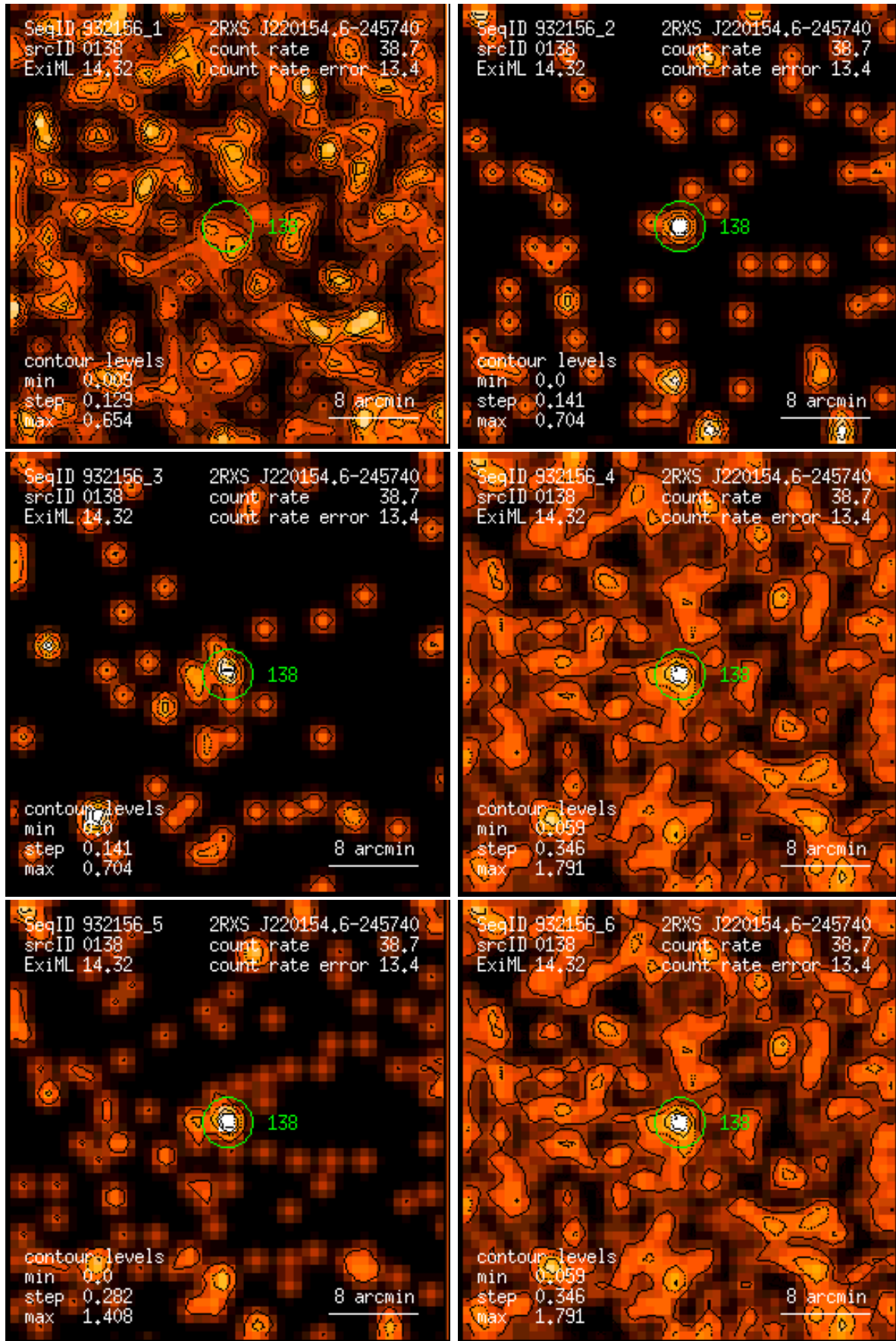
Figure 138: RASS 932156: detection 0138: band rate images, Gaussian filter: (1) PSPC channels 11 – 41, (2) 52 – 90, (3) 91 – 201, (4) 11 – 235, (5) 52 – 201, (6) 11 – 201. Broad band rates in counts/ks. Band rate contour levels in counts/ks/arcmin 2 .
