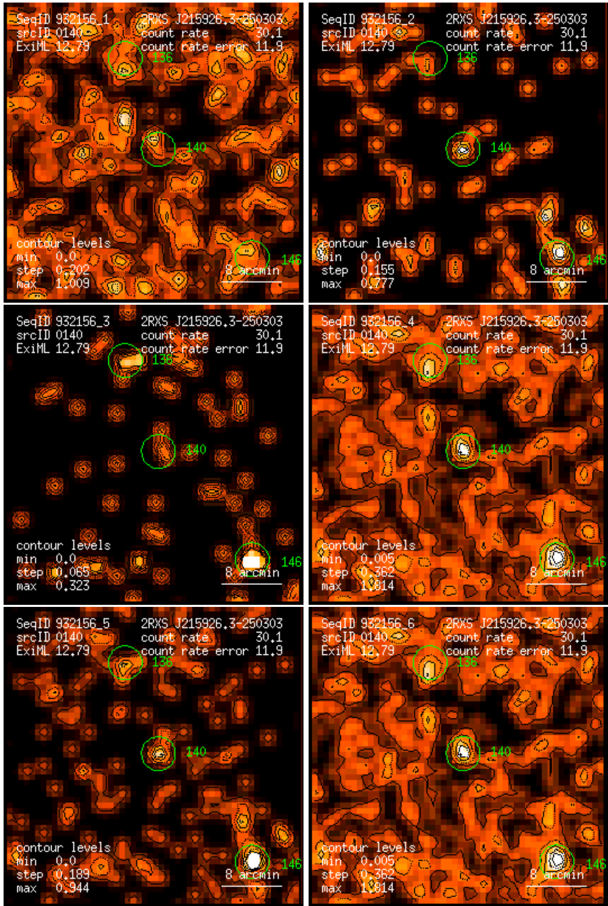
Figure 140: RASS 932156: detection 0140: band rate images, Gaussian filter: (1) PSPC channels 11 – 41, (2) 52 – 90, (3) 91 – 201, (4) 11 – 235, (5) 52 – 201, (6) 11 – 201. Broad band rates in counts/ks. Band rate contour levels in counts/ks/arcmin 2 .
