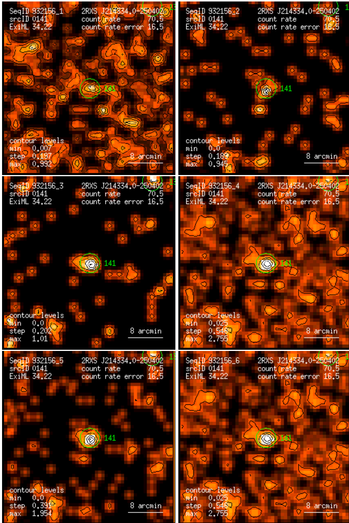
Figure 141: RASS 932156: detection 0141: band rate images, Gaussian filter: (1) PSPC channels 11 – 41, (2) 52 – 90, (3) 91 – 201, (4) 11 – 235, (5) 52 – 201, (6) 11 – 201. Broad band rates in counts/ks. Band rate contour levels in counts/ks/arcmin 2 .
