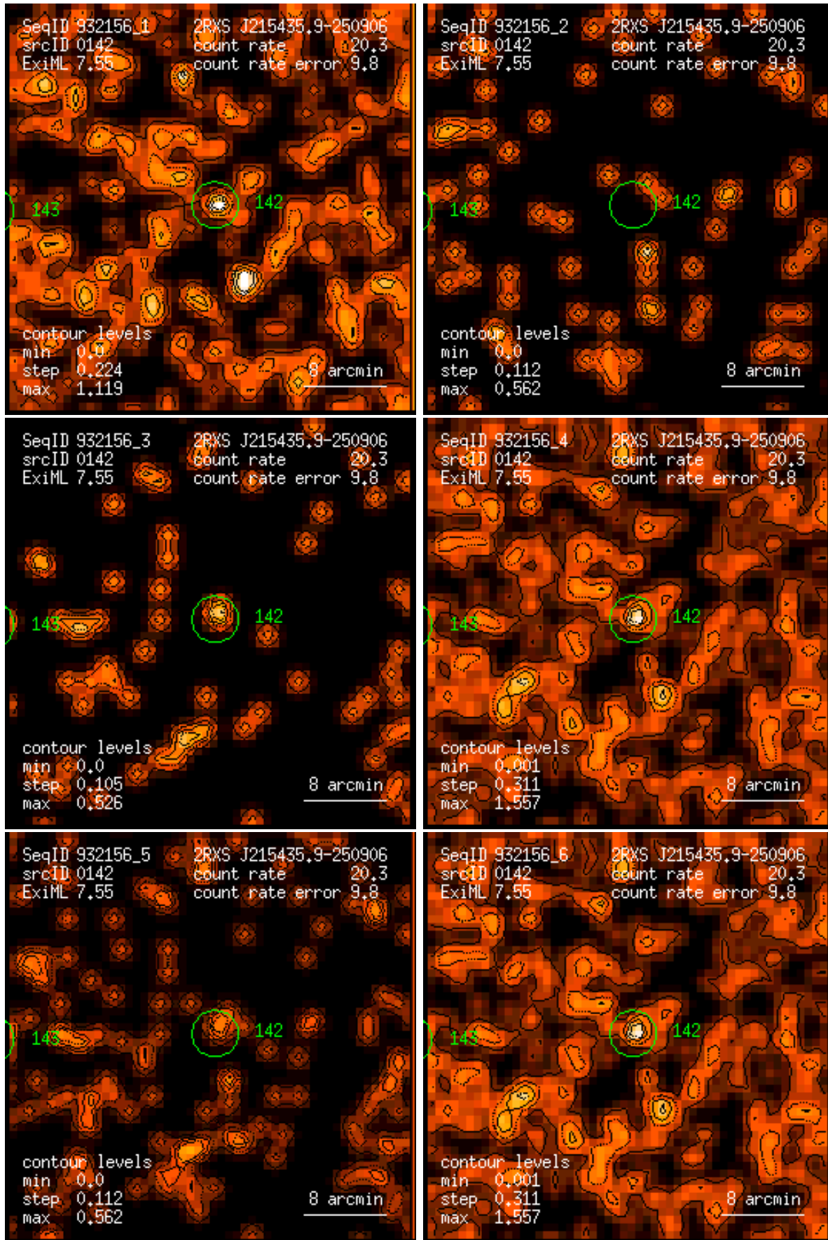
Figure 142: RASS 932156: detection 0142: band rate images, Gaussian filter: (1) PSPC channels 11 – 41, (2) 52 – 90, (3) 91 – 201, (4) 11 – 235, (5) 52 – 201, (6) 11 – 201. Broad band rates in counts/ks. Band rate contour levels in counts/ks/arcmin 2 .
