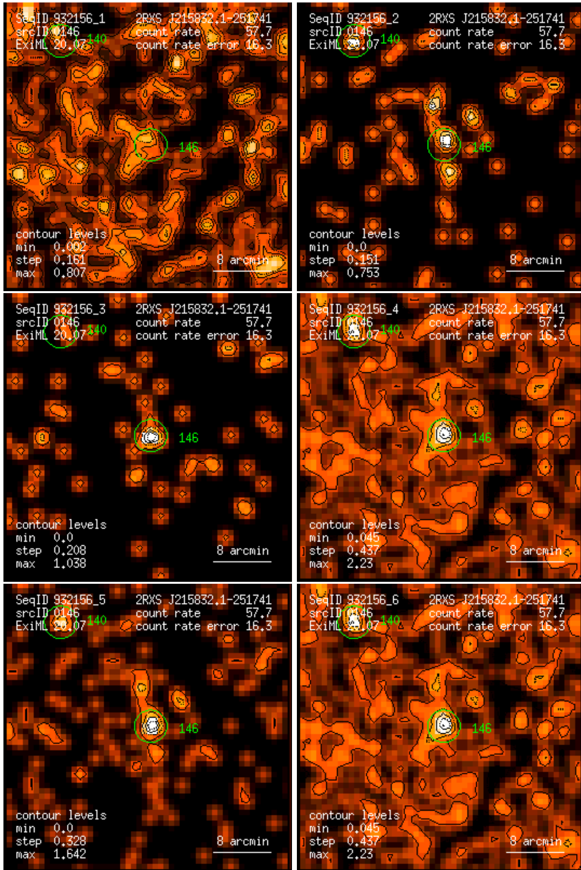
Figure 146: RASS 932156: detection 0146: band rate images, Gaussian filter: (1) PSPC channels 11 – 41, (2) 52 – 90, (3) 91 – 201, (4) 11 – 235, (5) 52 – 201, (6) 11 – 201. Broad band rates in counts/ks. Band rate contour levels in counts/ks/arcmin 2 .
