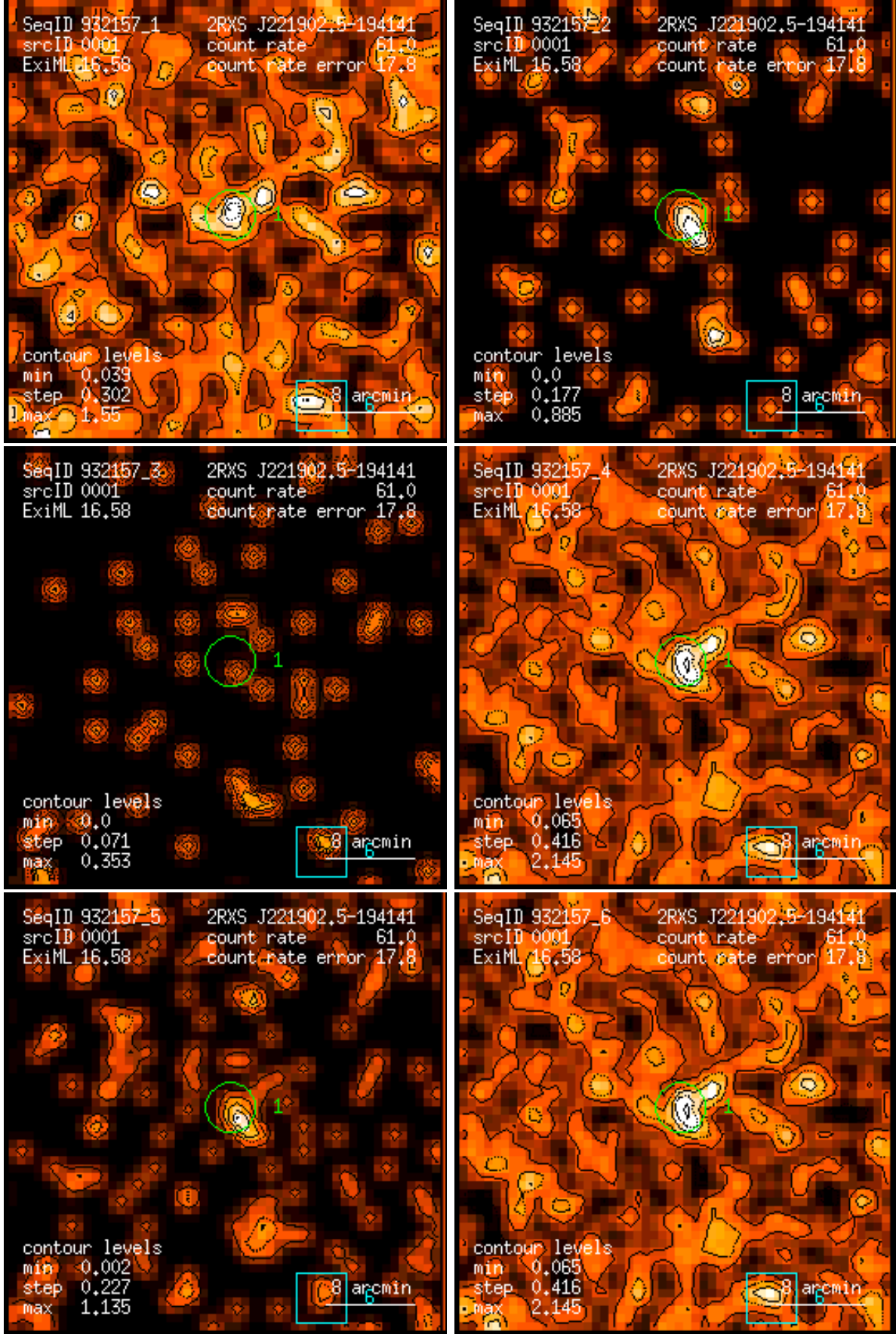
Figure 1: RASS 932157: detection 0001: band rate images, Gaussian filter: (1) PSPC channels 11 – 41, (2) 52 – 90, (3) 91 – 201, (4) 11 – 235, (5) 52 – 201, (6) 11 – 201. Broad band rates in counts/ks. Band rate contour levels in counts/ks/arcmin 2 .
