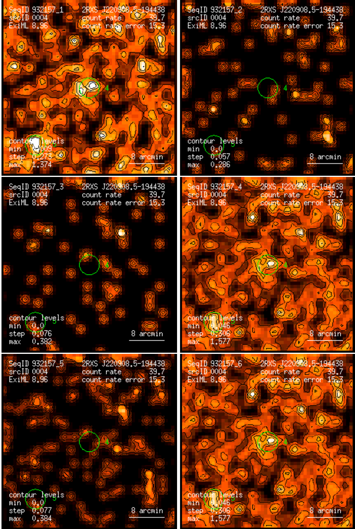
Figure 4: RASS 932157: detection 0004: band rate images, Gaussian filter: (1) PSPC channels 11 – 41, (2) 52 – 90, (3) 91 – 201, (4) 11 – 235, (5) 52 – 201, (6) 11 – 201. Broad band rates in counts/ks. Band rate contour levels in counts/ks/arcmin 2 .
