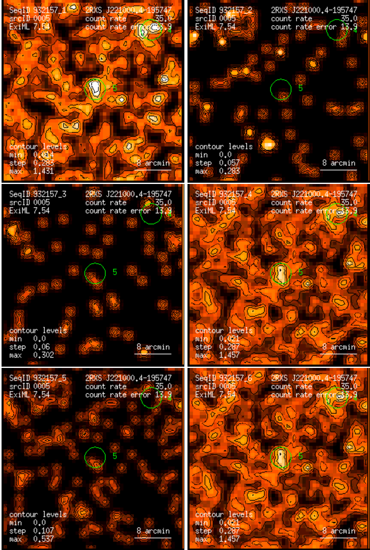
Figure 5: RASS 932157: detection 0005: band rate images, Gaussian filter: (1) PSPC channels 11 – 41, (2) 52 – 90, (3) 91 – 201, (4) 11 – 235, (5) 52 – 201, (6) 11 – 201. Broad band rates in counts/ks. Band rate contour levels in counts/ks/arcmin 2 .
