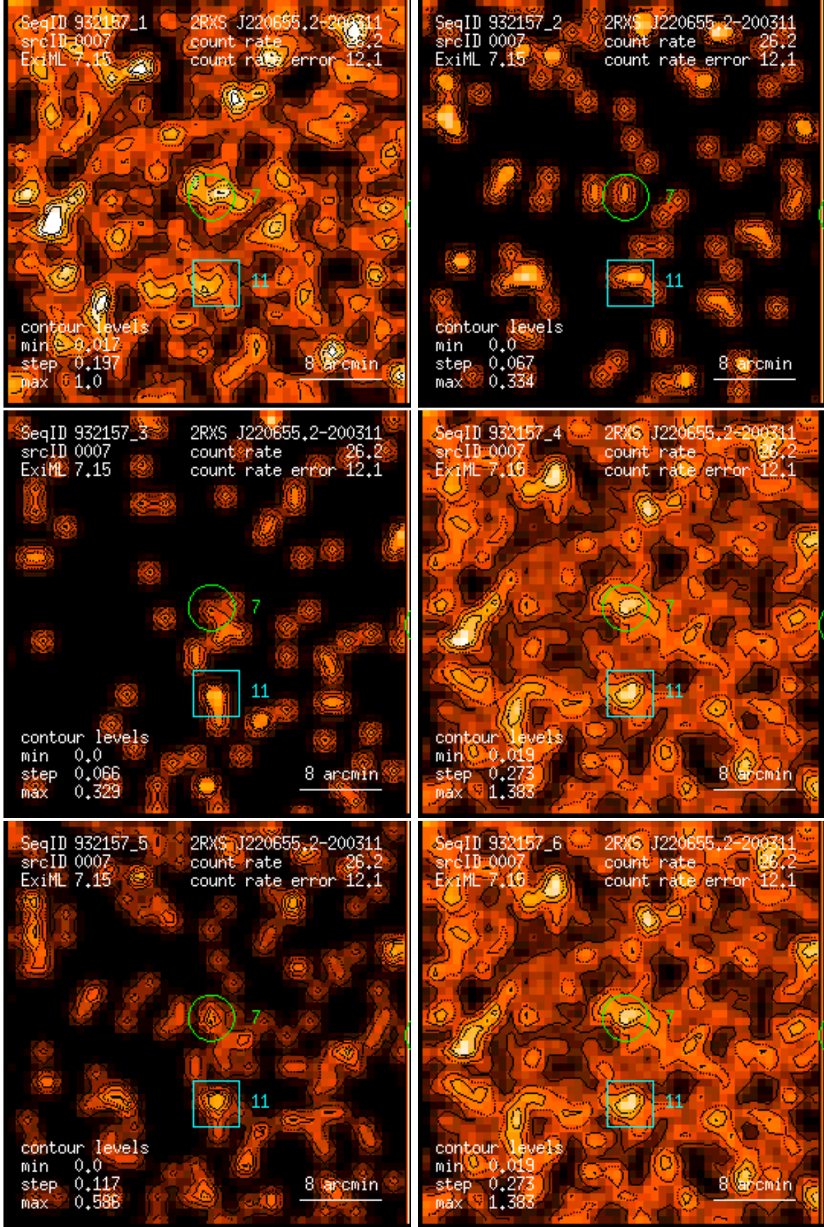
Figure 7: RASS 932157: detection 0007: band rate images, Gaussian filter: (1) PSPC channels 11 – 41, (2) 52 – 90, (3) 91 – 201, (4) 11 – 235, (5) 52 – 201, (6) 11 – 201. Broad band rates in counts/ks. Band rate contour levels in counts/ks/arcmin 2 .
