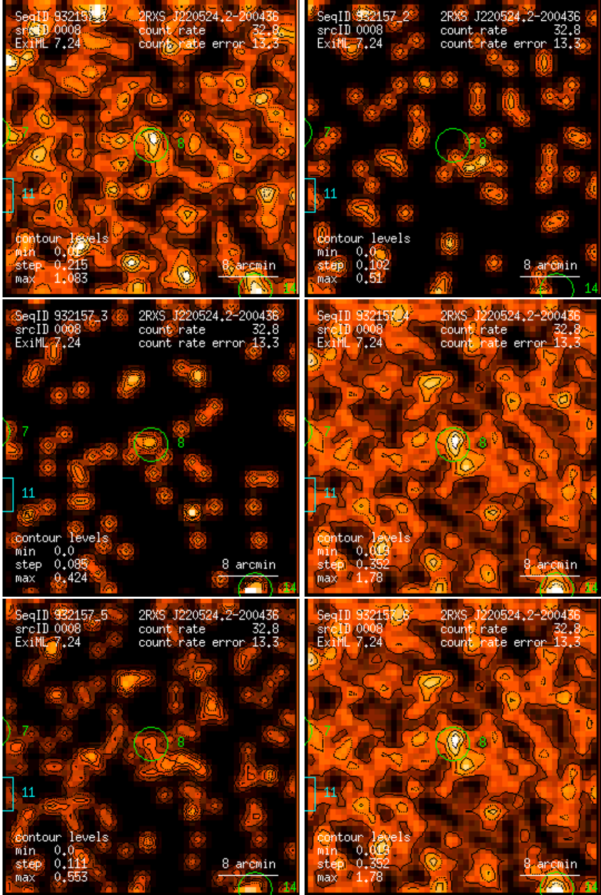
Figure 8: RASS 932157: detection 0008: band rate images, Gaussian filter: (1) PSPC channels 11 – 41, (2) 52 – 90, (3) 91 – 201, (4) 11 – 235, (5) 52 – 201, (6) 11 – 201. Broad band rates in counts/ks. Band rate contour levels in counts/ks/arcmin 2 .
