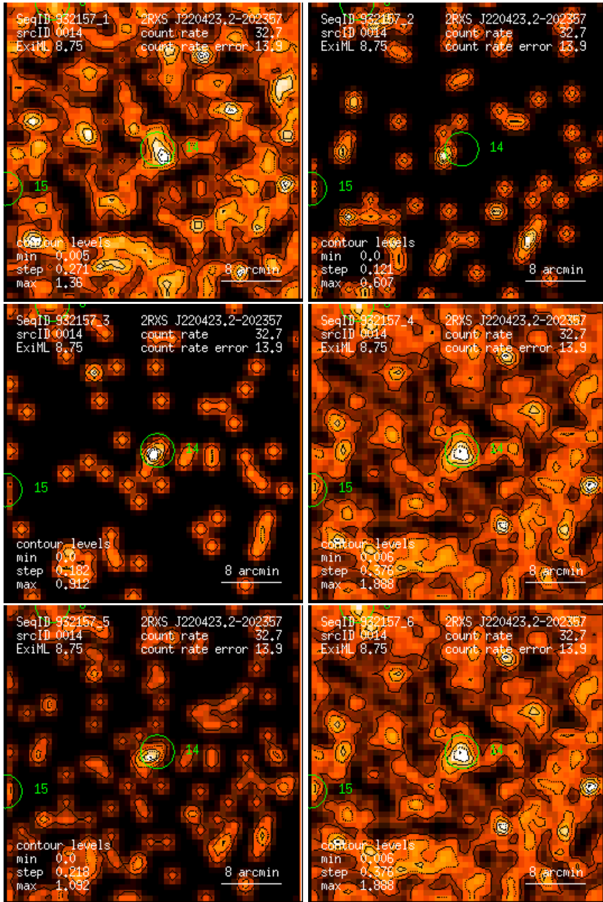
Figure 14: RASS 932157: detection 0014: band rate images, Gaussian filter: (1) PSPC channels 11 – 41, (2) 52 – 90, (3) 91 – 201, (4) 11 – 235, (5) 52 – 201, (6) 11 – 201. Broad band rates in counts/ks. Band rate contour levels in counts/ks/arcmin 2 .
