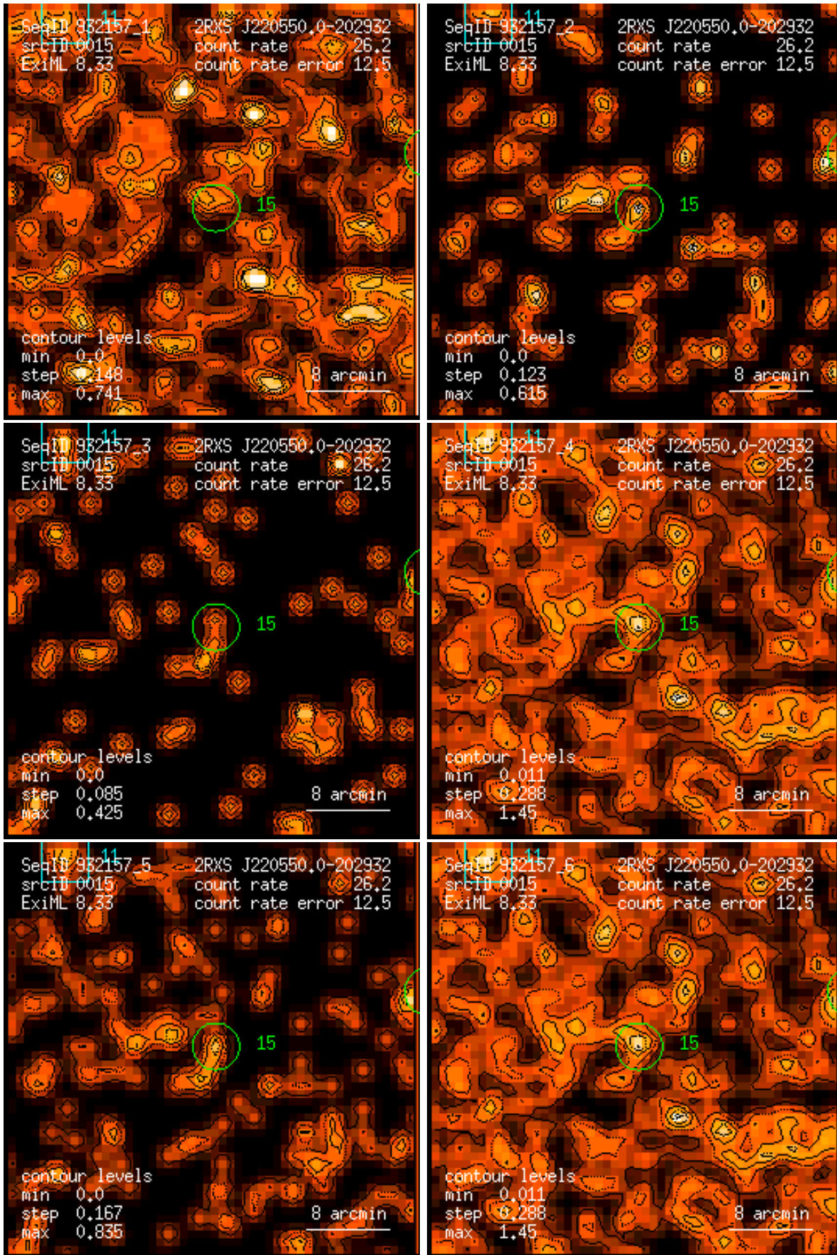
Figure 15: RASS 932157: detection 0015: band rate images, Gaussian filter: (1) PSPC channels 11 – 41, (2) 52 – 90, (3) 91 – 201, (4) 11 – 235, (5) 52 – 201, (6) 11 – 201. Broad band rates in counts/ks. Band rate contour levels in counts/ks/arcmin 2 .
