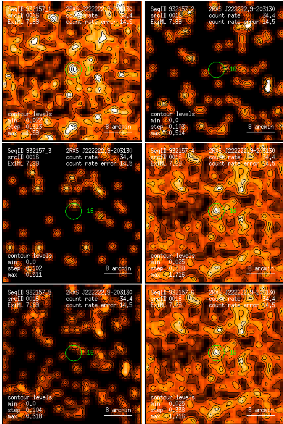
Figure 16: RASS 932157: detection 0016: band rate images, Gaussian filter: (1) PSPC channels 11 – 41, (2) 52 – 90, (3) 91 – 201, (4) 11 – 235, (5) 52 – 201, (6) 11 – 201. Broad band rates in counts/ks. Band rate contour levels in counts/ks/arcmin 2 .
