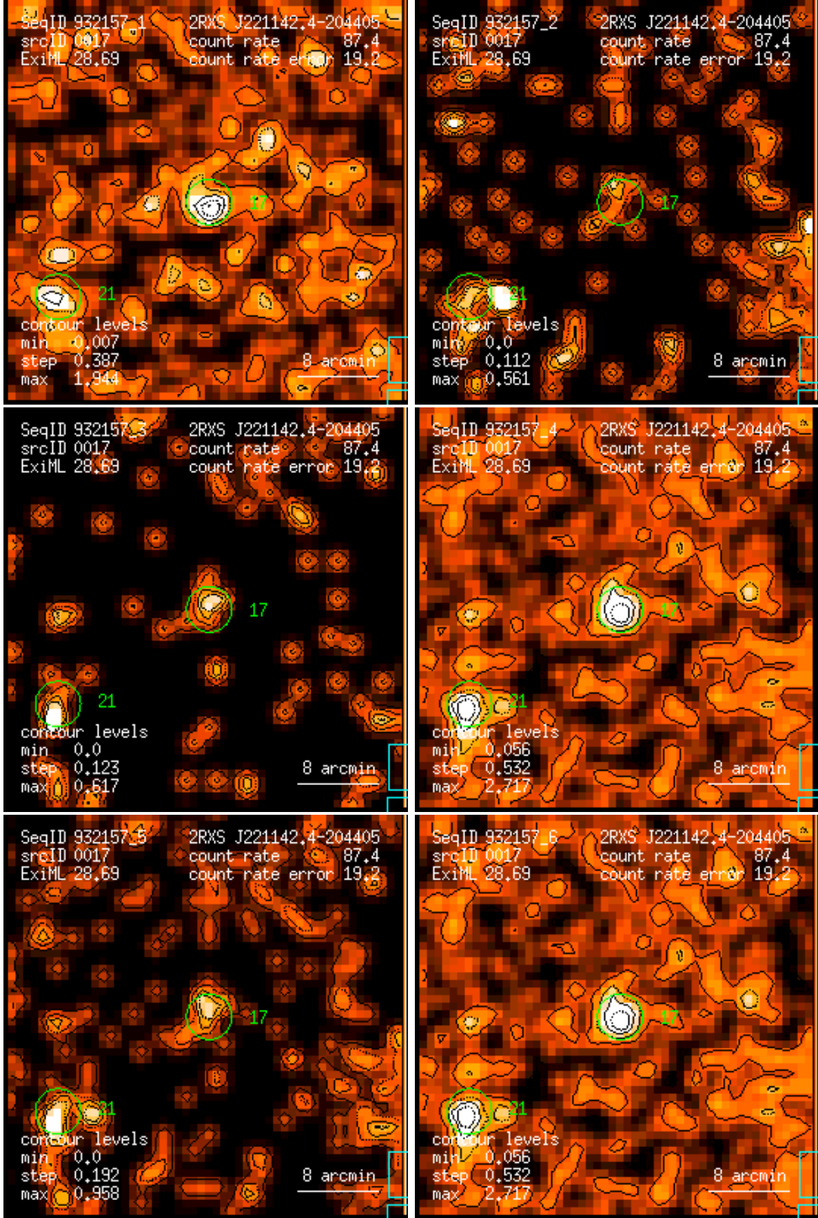
Figure 17: RASS 932157: detection 0017: band rate images, Gaussian filter: (1) PSPC channels 11 – 41, (2) 52 – 90, (3) 91 – 201, (4) 11 – 235, (5) 52 – 201, (6) 11 – 201. Broad band rates in counts/ks. Band rate contour levels in counts/ks/arcmin 2 .
