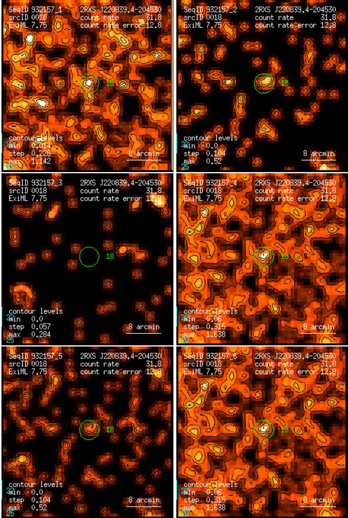
Figure 18: RASS 932157: detection 0018: band rate images, Gaussian filter: (1) PSPC channels 11 – 41, (2) 52 – 90, (3) 91 – 201, (4) 11 – 235, (5) 52 – 201, (6) 11 – 201. Broad band rates in counts/ks. Band rate contour levels in counts/ks/arcmin 2 .
