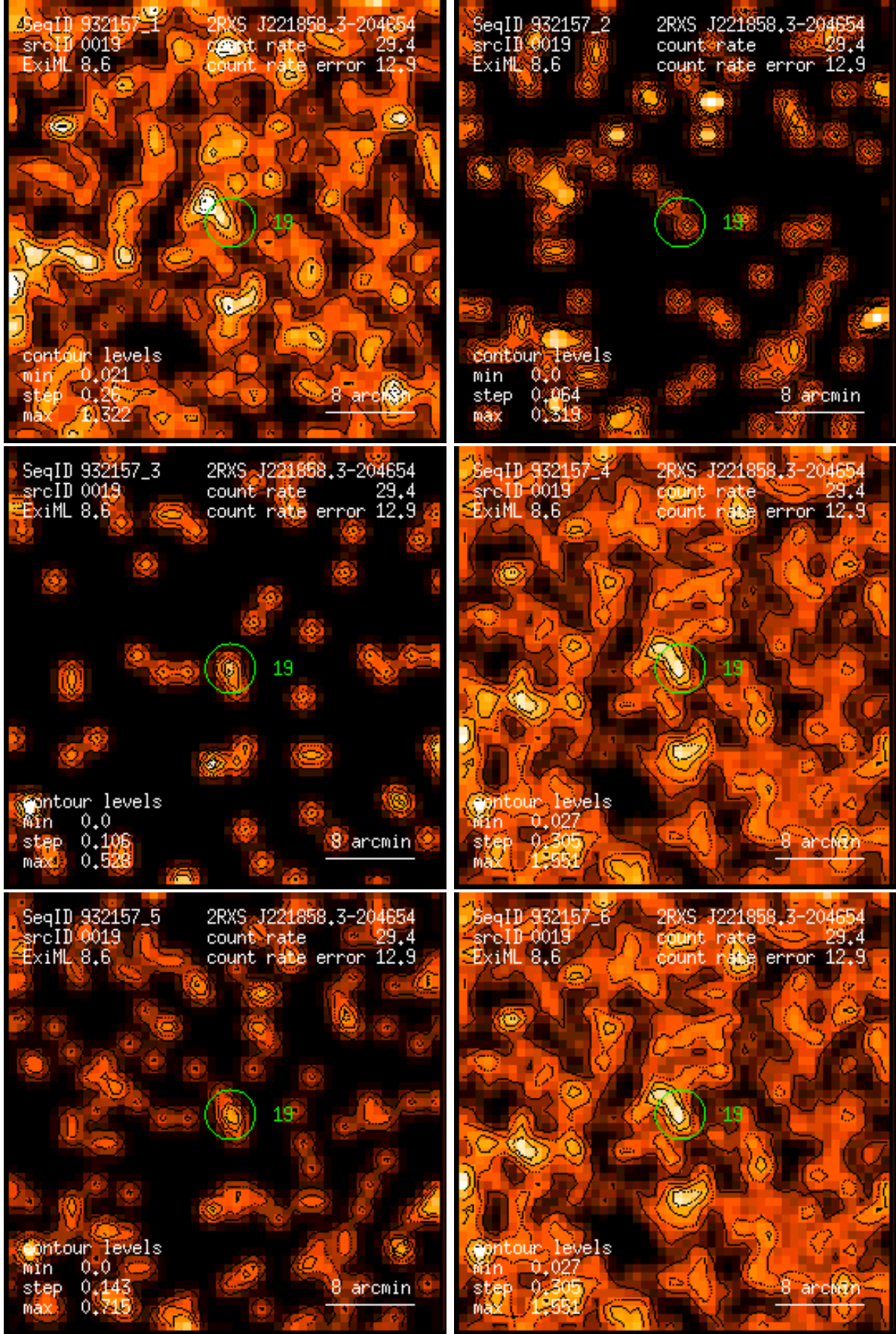
Figure 19: RASS 932157: detection 0019: band rate images, Gaussian filter: (1) PSPC channels 11 – 41, (2) 52 – 90, (3) 91 – 201, (4) 11 – 235, (5) 52 – 201, (6) 11 – 201. Broad band rates in counts/ks. Band rate contour levels in counts/ks/arcmin 2 .
