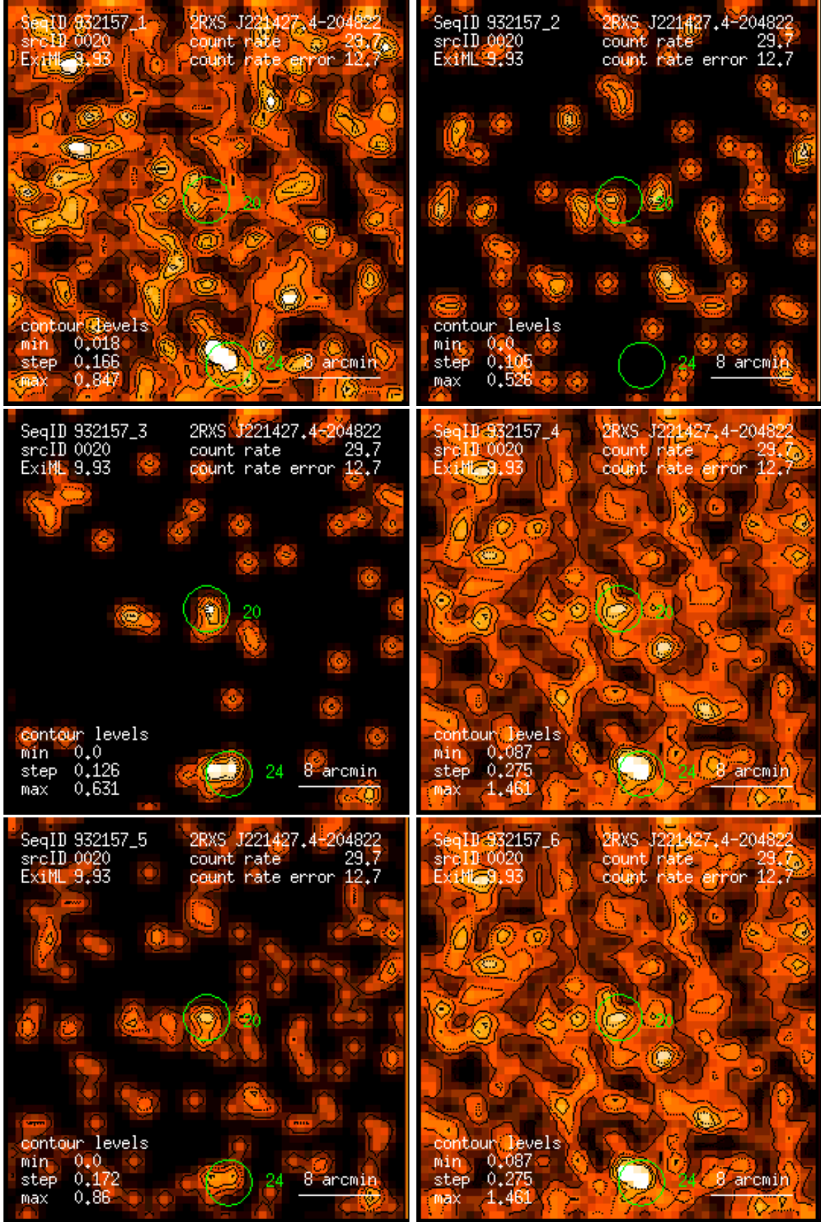
Figure 20: RASS 932157: detection 0020: band rate images, Gaussian filter: (1) PSPC channels 11 – 41, (2) 52 – 90, (3) 91 – 201, (4) 11 – 235, (5) 52 – 201, (6) 11 – 201. Broad band rates in counts/ks. Band rate contour levels in counts/ks/arcmin 2 .
