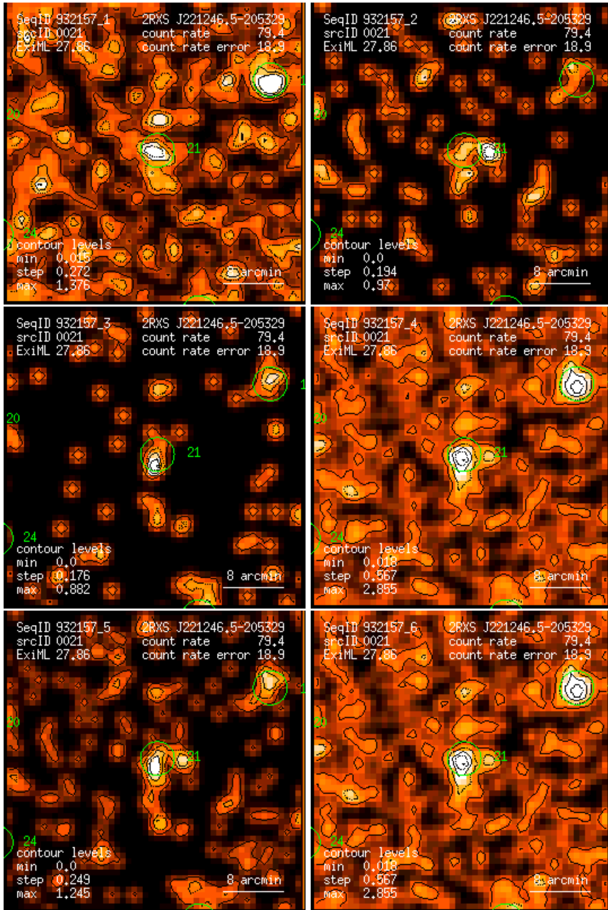
Figure 21: RASS 932157: detection 0021: band rate images, Gaussian filter: (1) PSPC channels 11 – 41, (2) 52 – 90, (3) 91 – 201, (4) 11 – 235, (5) 52 – 201, (6) 11 – 201. Broad band rates in counts/ks. Band rate contour levels in counts/ks/arcmin 2 .
