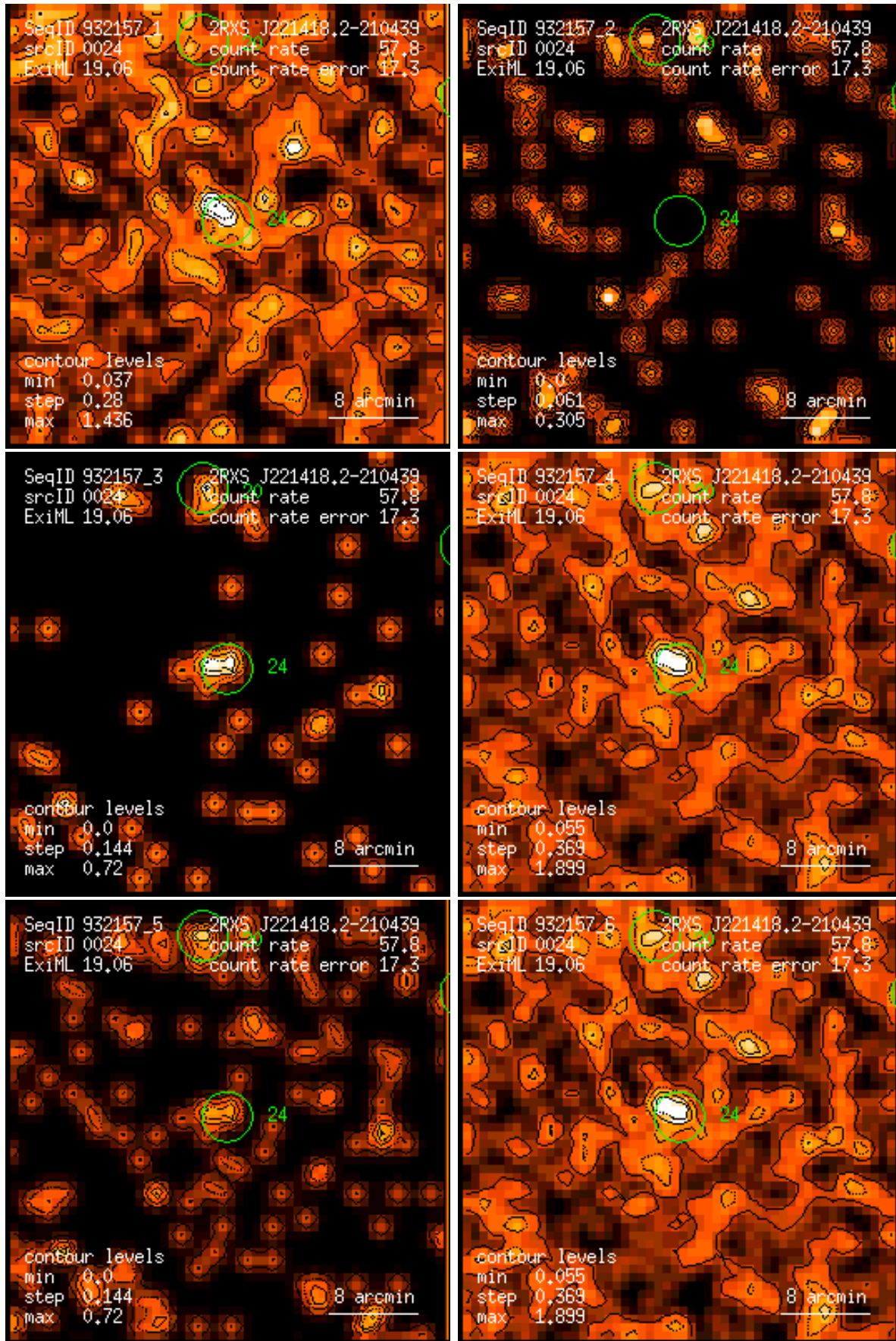
Figure 24: RASS 932157: detection 0024: band rate images, Gaussian filter: (1) PSPC channels 11 – 41, (2) 52 – 90, (3) 91 – 201, (4) 11 – 235, (5) 52 – 201, (6) 11 – 201. Broad band rates in counts/ks. Band rate contour levels in counts/ks/arcmin 2 .
