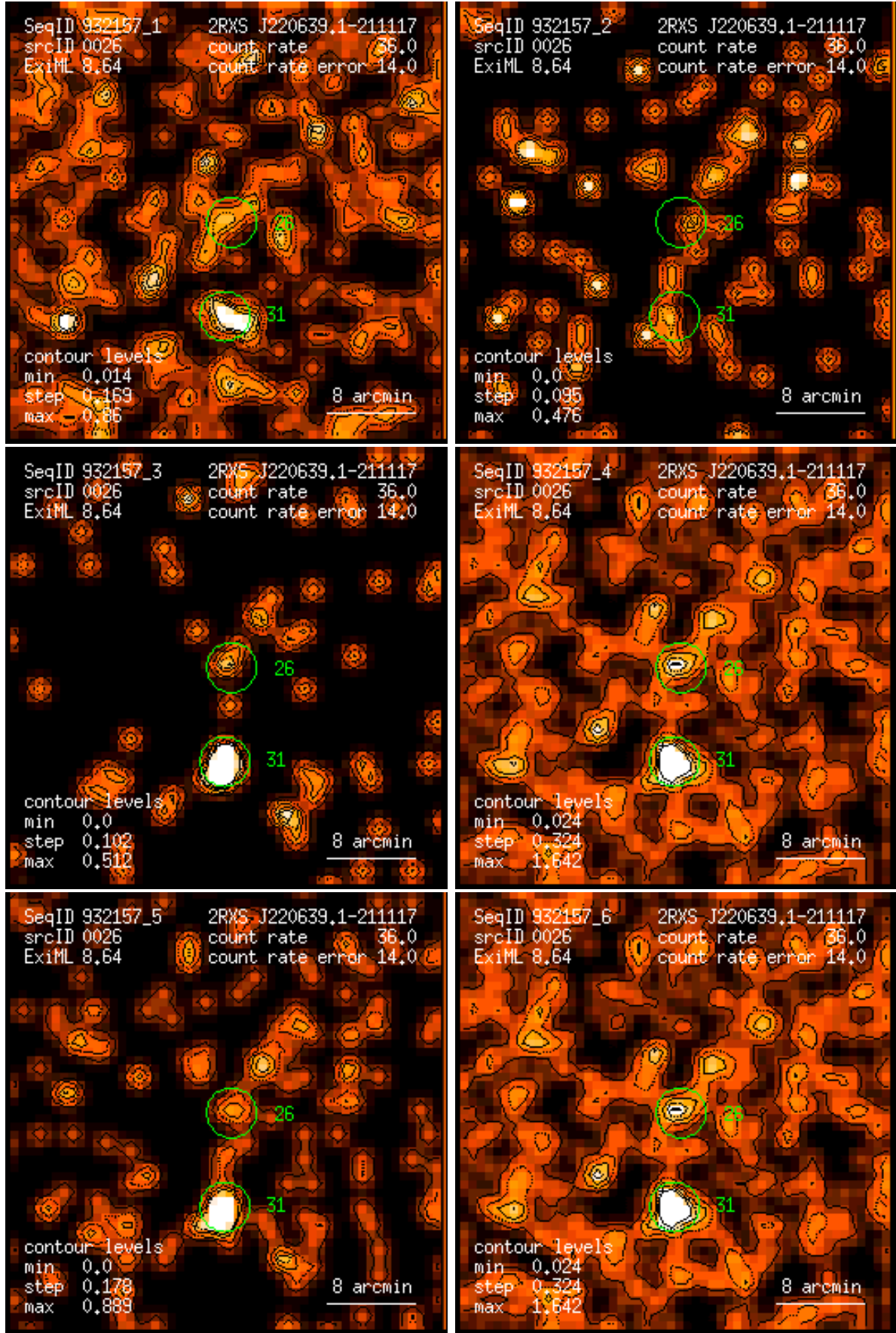
Figure 26: RASS 932157: detection 0026: band rate images, Gaussian filter: (1) PSPC channels 11 – 41, (2) 52 – 90, (3) 91 – 201, (4) 11 – 235, (5) 52 – 201, (6) 11 – 201. Broad band rates in counts/ks. Band rate contour levels in counts/ks/arcmin 2 .
