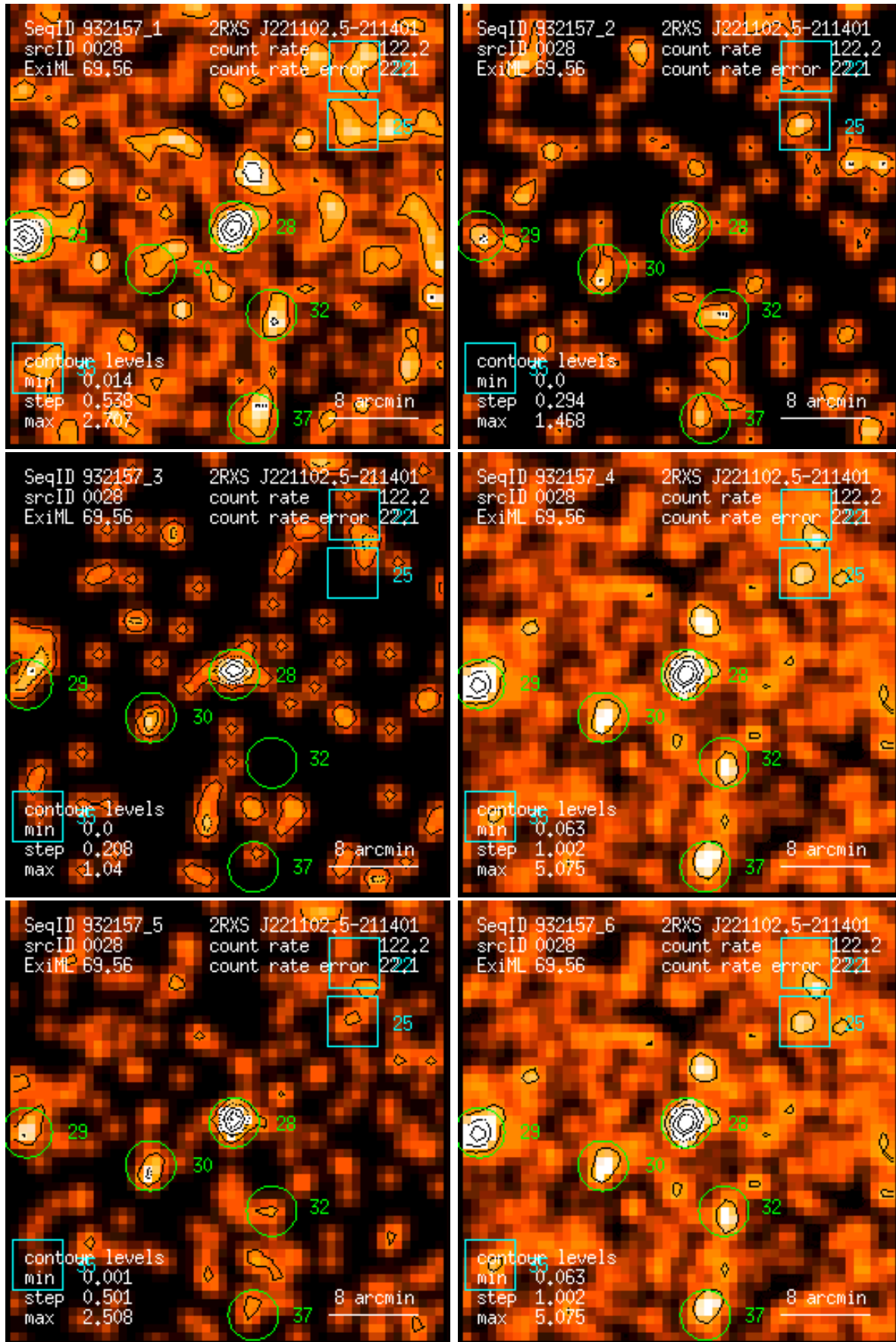
Figure 28: RASS 932157: detection 0028: band rate images, Gaussian filter: (1) PSPC channels 11 – 41, (2) 52 – 90, (3) 91 – 201, (4) 11 – 235, (5) 52 – 201, (6) 11 – 201. Broad band rates in counts/ks. Band rate contour levels in counts/ks/arcmin 2 .
