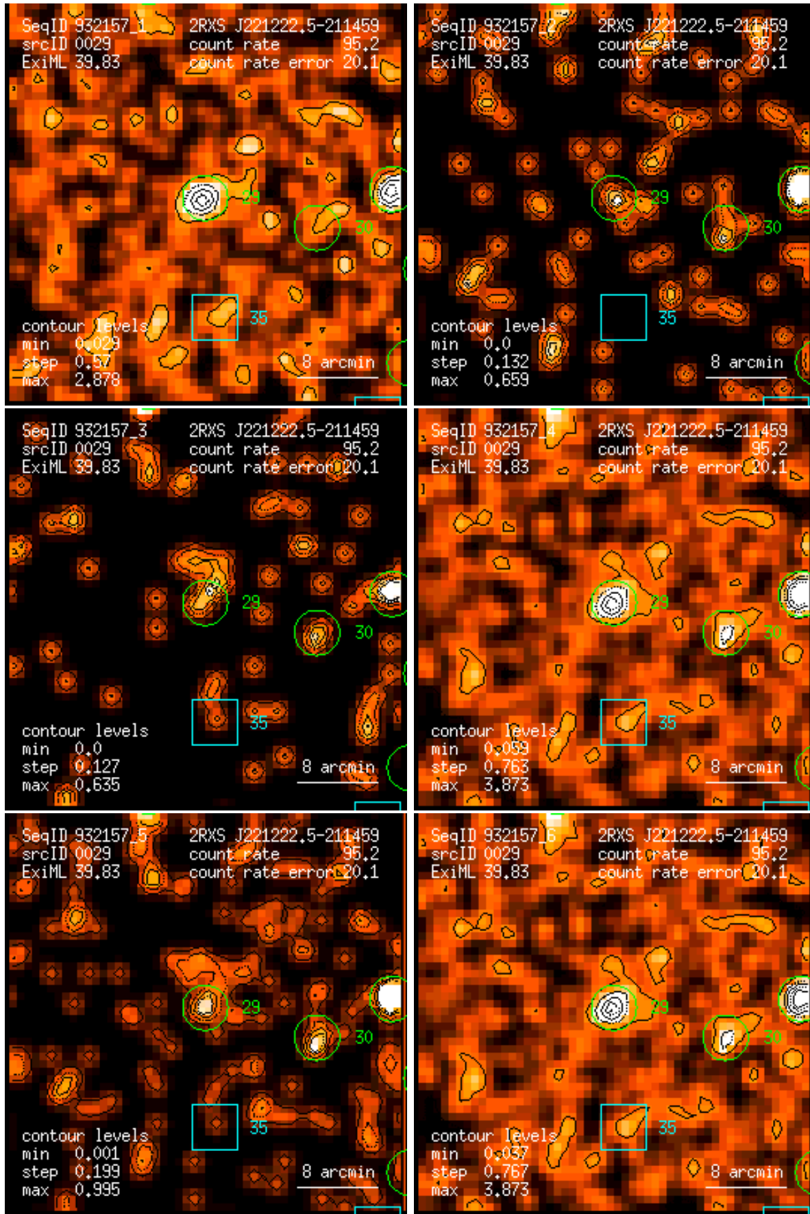
Figure 29: RASS 932157: detection 0029: band rate images, Gaussian filter: (1) PSPC channels 11 – 41, (2) 52 – 90, (3) 91 – 201, (4) 11 – 235, (5) 52 – 201, (6) 11 – 201. Broad band rates in counts/ks. Band rate contour levels in counts/ks/arcmin 2 .
