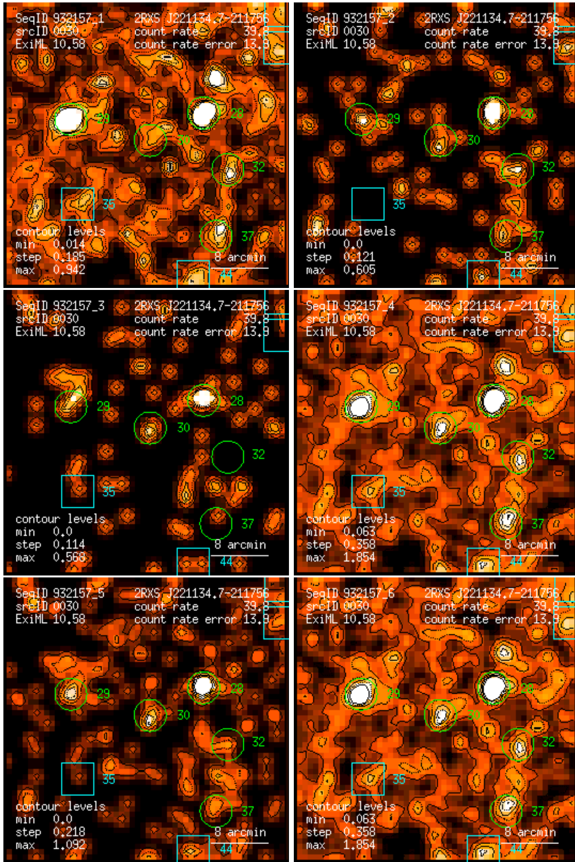
Figure 30: RASS 932157: detection 0030: band rate images, Gaussian filter: (1) PSPC channels 11 – 41, (2) 52 – 90, (3) 91 – 201, (4) 11 – 235, (5) 52 – 201, (6) 11 – 201. Broad band rates in counts/ks. Band rate contour levels in counts/ks/arcmin 2 .
