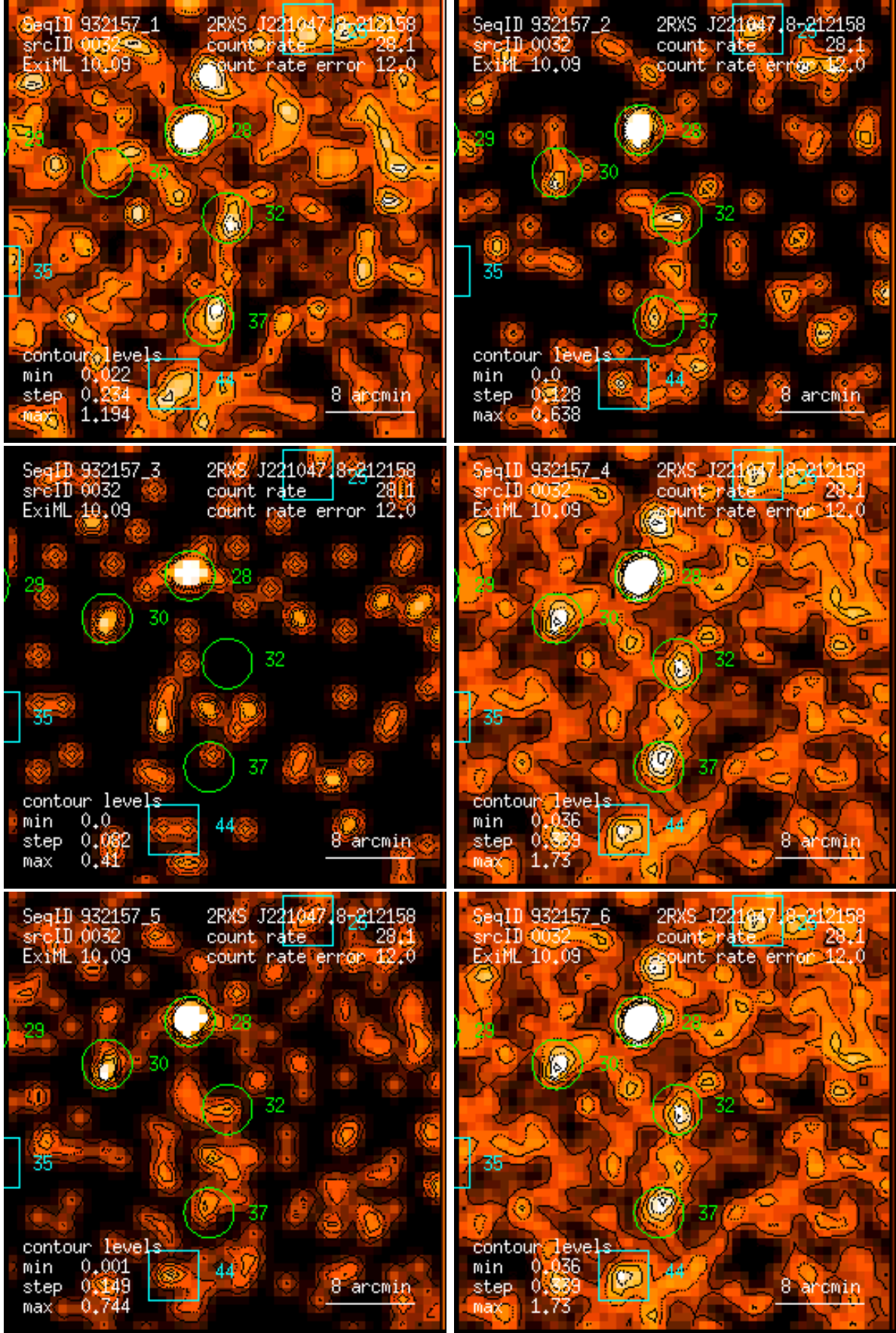
Figure 32: RASS 932157: detection 0032: band rate images, Gaussian filter: (1) PSPC channels 11 – 41, (2) 52 – 90, (3) 91 – 201, (4) 11 – 235, (5) 52 – 201, (6) 11 – 201. Broad band rates in counts/ks. Band rate contour levels in counts/ks/arcmin 2 .
