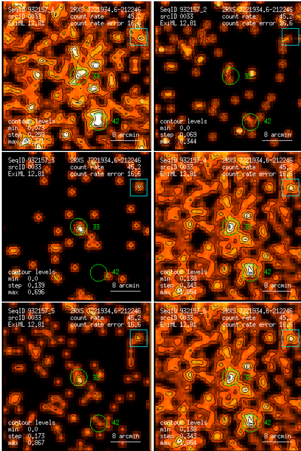
Figure 33: RASS 932157: detection 0033: band rate images, Gaussian filter: (1) PSPC channels 11 – 41, (2) 52 – 90, (3) 91 – 201, (4) 11 – 235, (5) 52 – 201, (6) 11 – 201. Broad band rates in counts/ks. Band rate contour levels in counts/ks/arcmin 2 .
