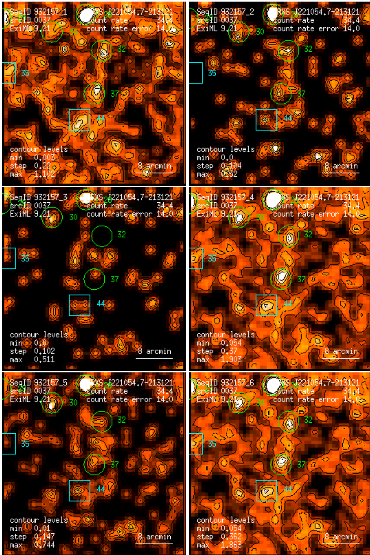
Figure 37: RASS 932157: detection 0037: band rate images, Gaussian filter: (1) PSPC channels 11 – 41, (2) 52 – 90, (3) 91 – 201, (4) 11 – 235, (5) 52 – 201, (6) 11 – 201. Broad band rates in counts/ks. Band rate contour levels in counts/ks/arcmin 2 .
