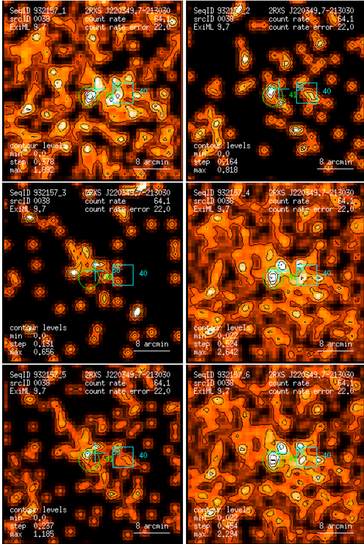
Figure 38: RASS 932157: detection 0038: band rate images, Gaussian filter: (1) PSPC channels 11 – 41, (2) 52 – 90, (3) 91 – 201, (4) 11 – 235, (5) 52 – 201, (6) 11 – 201. Broad band rates in counts/ks. Band rate contour levels in counts/ks/arcmin 2 .
