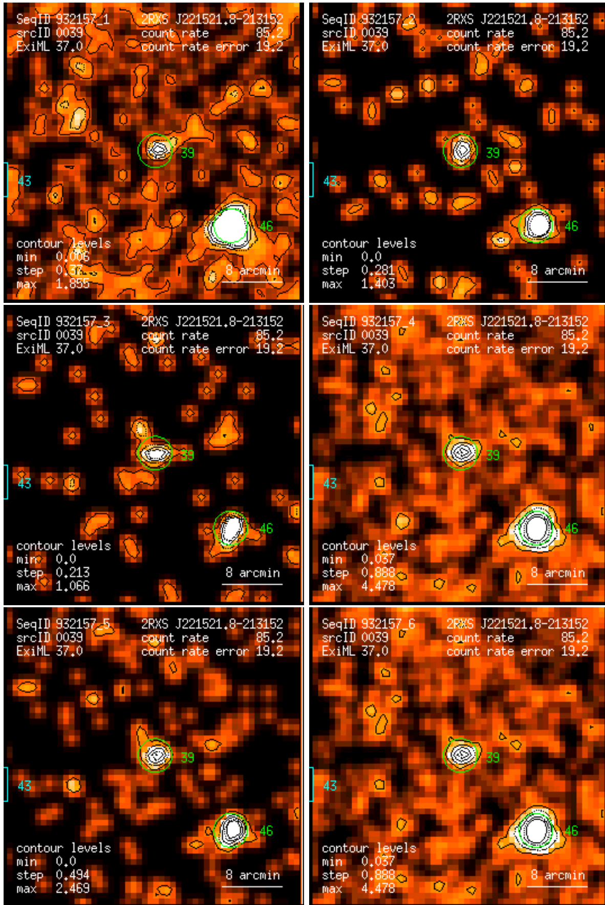
Figure 39: RASS 932157: detection 0039: band rate images, Gaussian filter: (1) PSPC channels 11 – 41, (2) 52 – 90, (3) 91 – 201, (4) 11 – 235, (5) 52 – 201, (6) 11 – 201. Broad band rates in counts/ks. Band rate contour levels in counts/ks/arcmin 2 .
