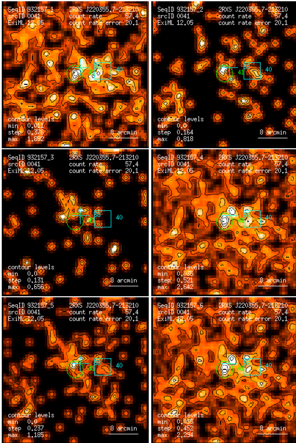
Figure 41: RASS 932157: detection 0041: band rate images, Gaussian filter: (1) PSPC channels 11 – 41, (2) 52 – 90, (3) 91 – 201, (4) 11 – 235, (5) 52 – 201, (6) 11 – 201. Broad band rates in counts/ks. Band rate contour levels in counts/ks/arcmin 2 .
