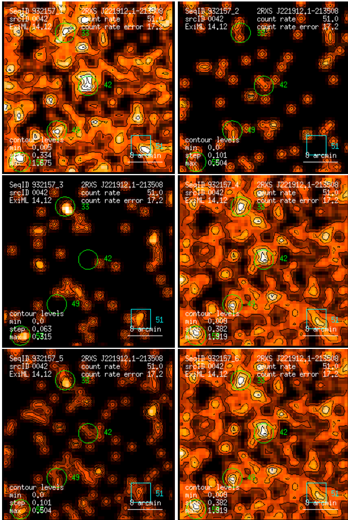
Figure 42: RASS 932157: detection 0042: band rate images, Gaussian filter: (1) PSPC channels 11 – 41, (2) 52 – 90, (3) 91 – 201, (4) 11 – 235, (5) 52 – 201, (6) 11 – 201. Broad band rates in counts/ks. Band rate contour levels in counts/ks/arcmin 2 .
