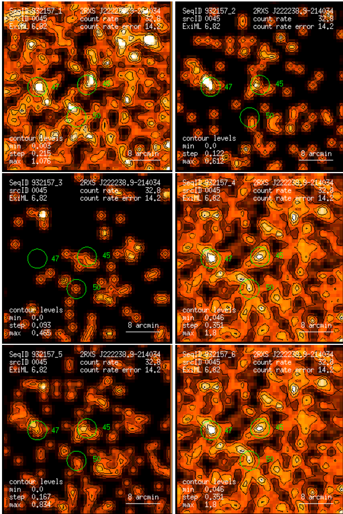
Figure 45: RASS 932157: detection 0045: band rate images, Gaussian filter: (1) PSPC channels 11 – 41, (2) 52 – 90, (3) 91 – 201, (4) 11 – 235, (5) 52 – 201, (6) 11 – 201. Broad band rates in counts/ks. Band rate contour levels in counts/ks/arcmin 2 .
