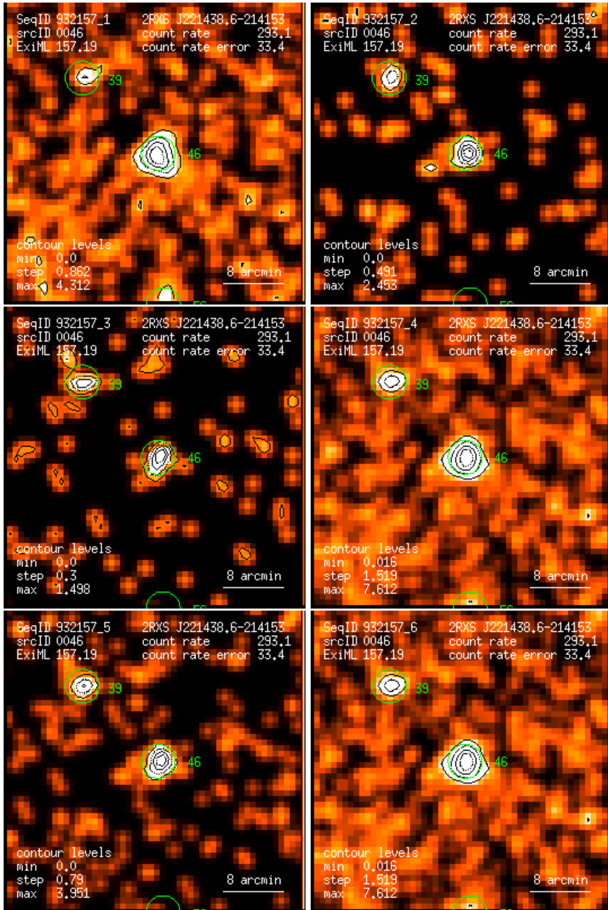
Figure 46: RASS 932157: detection 0046: band rate images, Gaussian filter: (1) PSPC channels 11 – 41, (2) 52 – 90, (3) 91 – 201, (4) 11 – 235, (5) 52 – 201, (6) 11 – 201. Broad band rates in counts/ks. Band rate contour levels in counts/ks/arcmin 2 .
