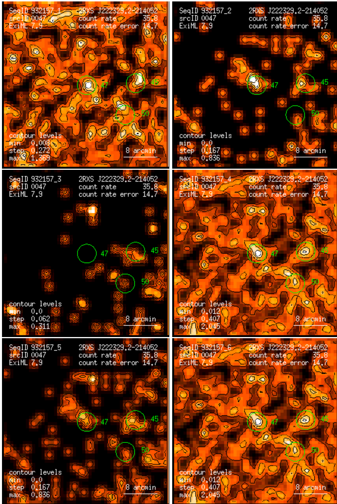
Figure 47: RASS 932157: detection 0047: band rate images, Gaussian filter: (1) PSPC channels 11 – 41, (2) 52 – 90, (3) 91 – 201, (4) 11 – 235, (5) 52 – 201, (6) 11 – 201. Broad band rates in counts/ks. Band rate contour levels in counts/ks/arcmin 2 .
