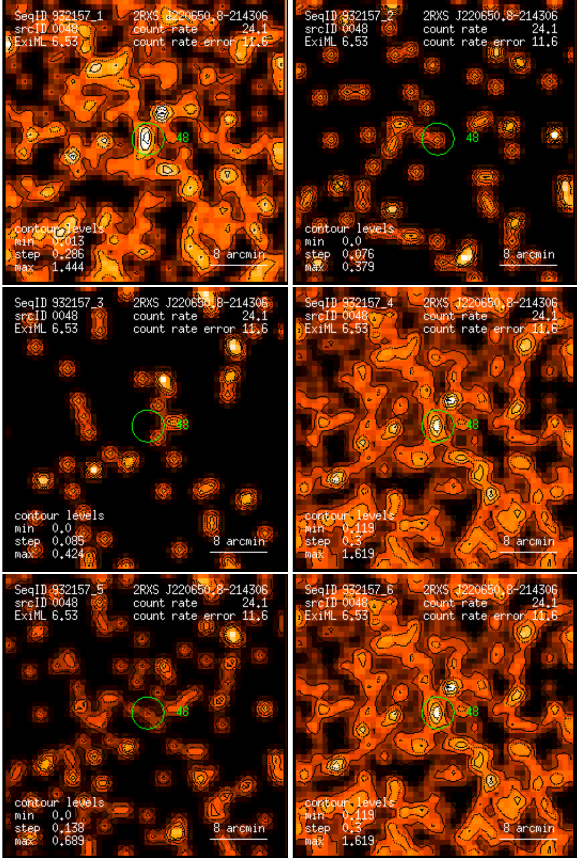
Figure 48: RASS 932157: detection 0048: band rate images, Gaussian filter: (1) PSPC channels 11 – 41, (2) 52 – 90, (3) 91 – 201, (4) 11 – 235, (5) 52 – 201, (6) 11 – 201. Broad band rates in counts/ks. Band rate contour levels in counts/ks/arcmin 2 .
