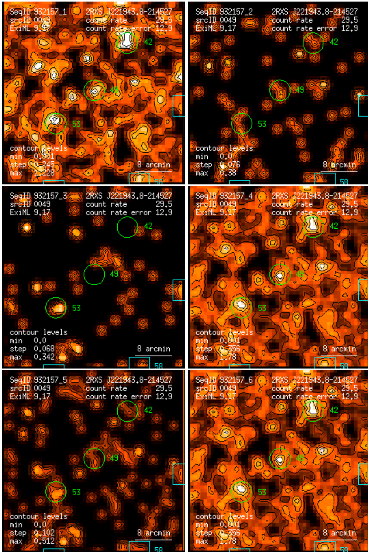
Figure 49: RASS 932157: detection 0049: band rate images, Gaussian filter: (1) PSPC channels 11 – 41, (2) 52 – 90, (3) 91 – 201, (4) 11 – 235, (5) 52 – 201, (6) 11 – 201. Broad band rates in counts/ks. Band rate contour levels in counts/ks/arcmin 2 .
