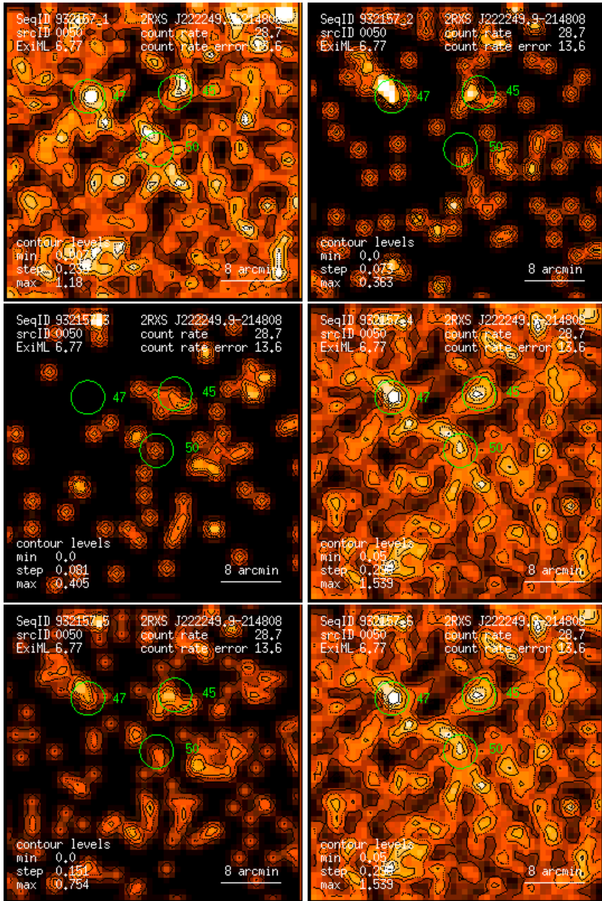
Figure 50: RASS 932157: detection 0050: band rate images, Gaussian filter: (1) PSPC channels 11 – 41, (2) 52 – 90, (3) 91 – 201, (4) 11 – 235, (5) 52 – 201, (6) 11 – 201. Broad band rates in counts/ks. Band rate contour levels in counts/ks/arcmin 2 .
