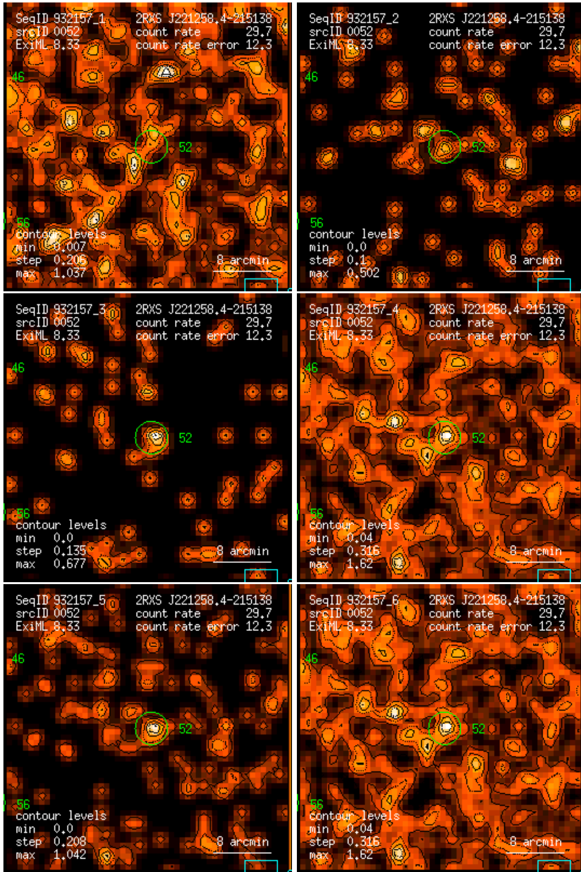
Figure 52: RASS 932157: detection 0052: band rate images, Gaussian filter: (1) PSPC channels 11 – 41, (2) 52 – 90, (3) 91 – 201, (4) 11 – 235, (5) 52 – 201, (6) 11 – 201. Broad band rates in counts/ks. Band rate contour levels in counts/ks/arcmin 2 .
