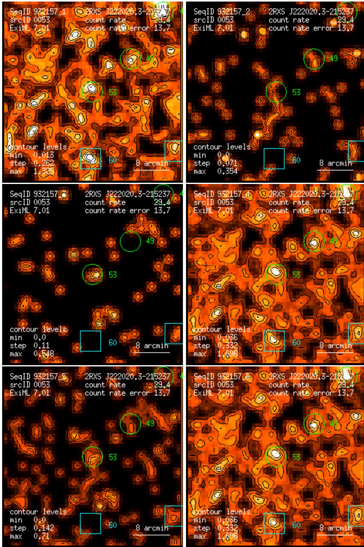
Figure 53: RASS 932157: detection 0053: band rate images, Gaussian filter: (1) PSPC channels 11 – 41, (2) 52 – 90, (3) 91 – 201, (4) 11 – 235, (5) 52 – 201, (6) 11 – 201. Broad band rates in counts/ks. Band rate contour levels in counts/ks/arcmin 2 .
