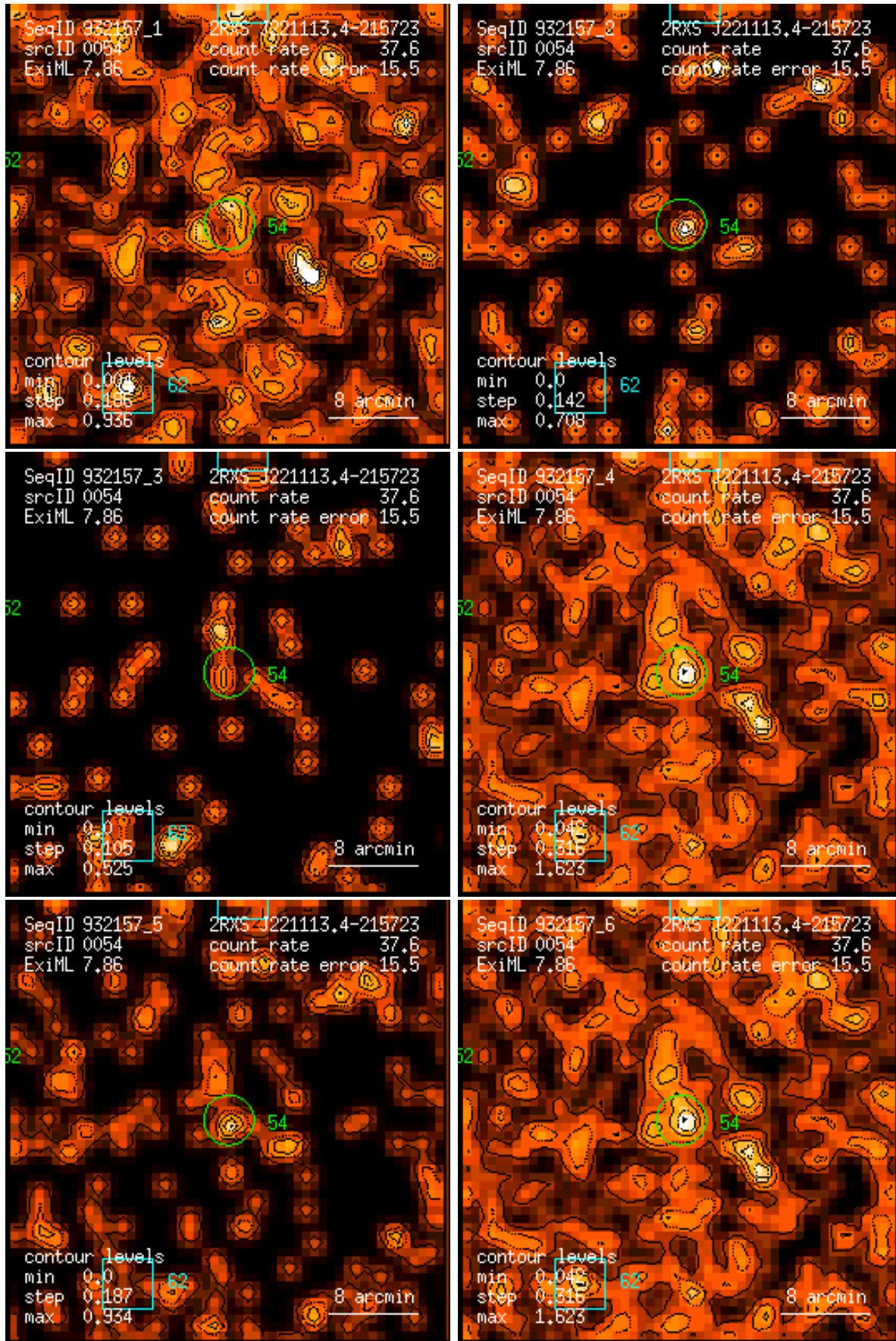
Figure 54: RASS 932157: detection 0054: band rate images, Gaussian filter: (1) PSPC channels 11 – 41, (2) 52 – 90, (3) 91 – 201, (4) 11 – 235, (5) 52 – 201, (6) 11 – 201. Broad band rates in counts/ks. Band rate contour levels in counts/ks/arcmin 2 .
