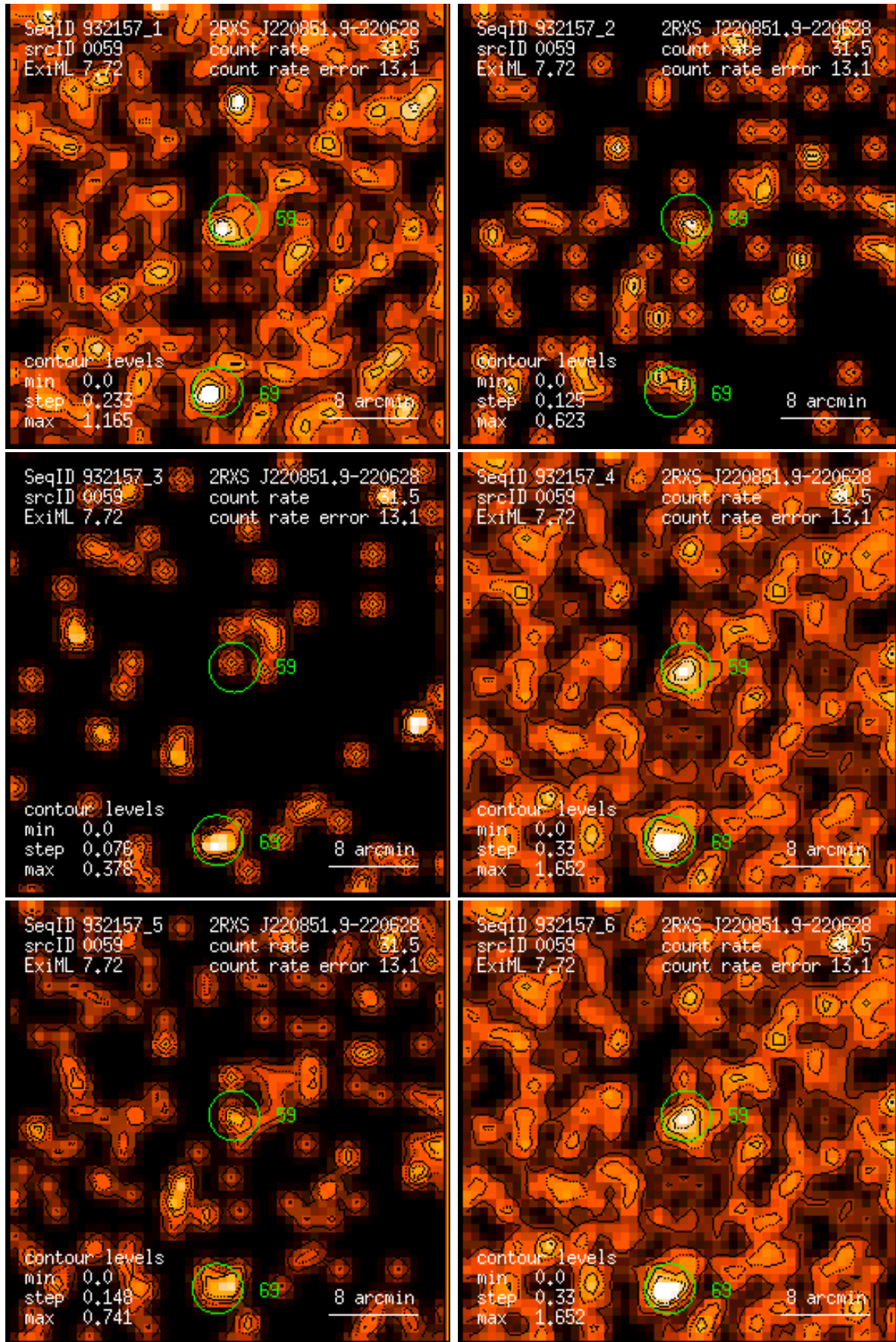
Figure 59: RASS 932157: detection 0059: band rate images, Gaussian filter: (1) PSPC channels 11 – 41, (2) 52 – 90, (3) 91 – 201, (4) 11 – 235, (5) 52 – 201, (6) 11 – 201. Broad band rates in counts/ks. Band rate contour levels in counts/ks/arcmin 2 .
