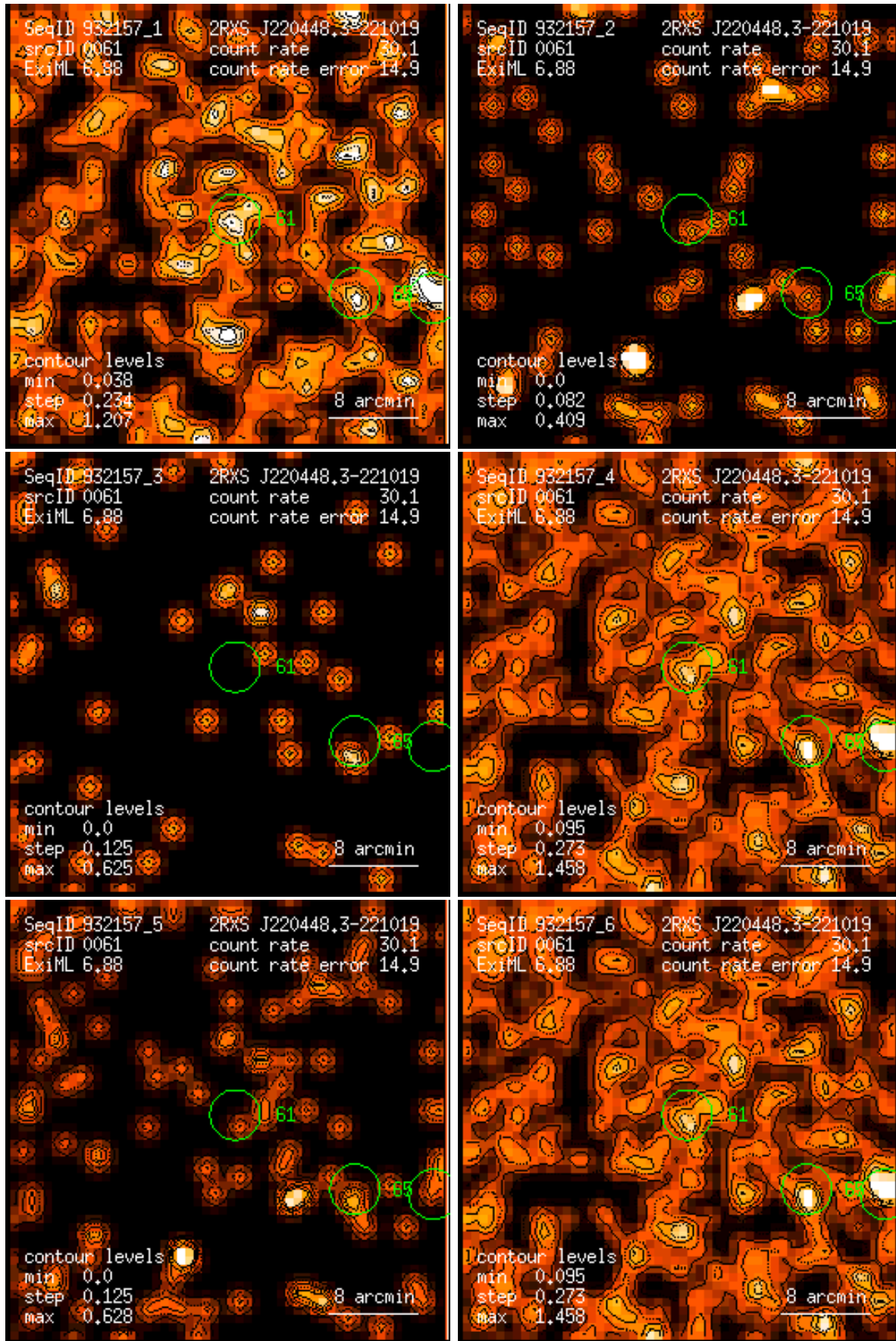
Figure 61: RASS 932157: detection 0061: band rate images, Gaussian filter: (1) PSPC channels 11 – 41, (2) 52 – 90, (3) 91 – 201, (4) 11 – 235, (5) 52 – 201, (6) 11 – 201. Broad band rates in counts/ks. Band rate contour levels in counts/ks/arcmin 2 .
