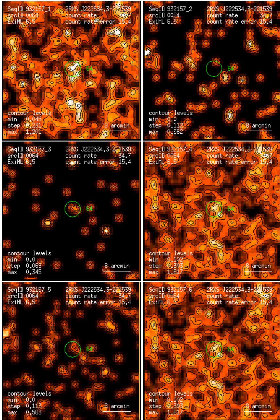
Figure 64: RASS 932157: detection 0064: band rate images, Gaussian filter: (1) PSPC channels 11 – 41, (2) 52 – 90, (3) 91 – 201, (4) 11 – 235, (5) 52 – 201, (6) 11 – 201. Broad band rates in counts/ks. Band rate contour levels in counts/ks/arcmin 2 .
