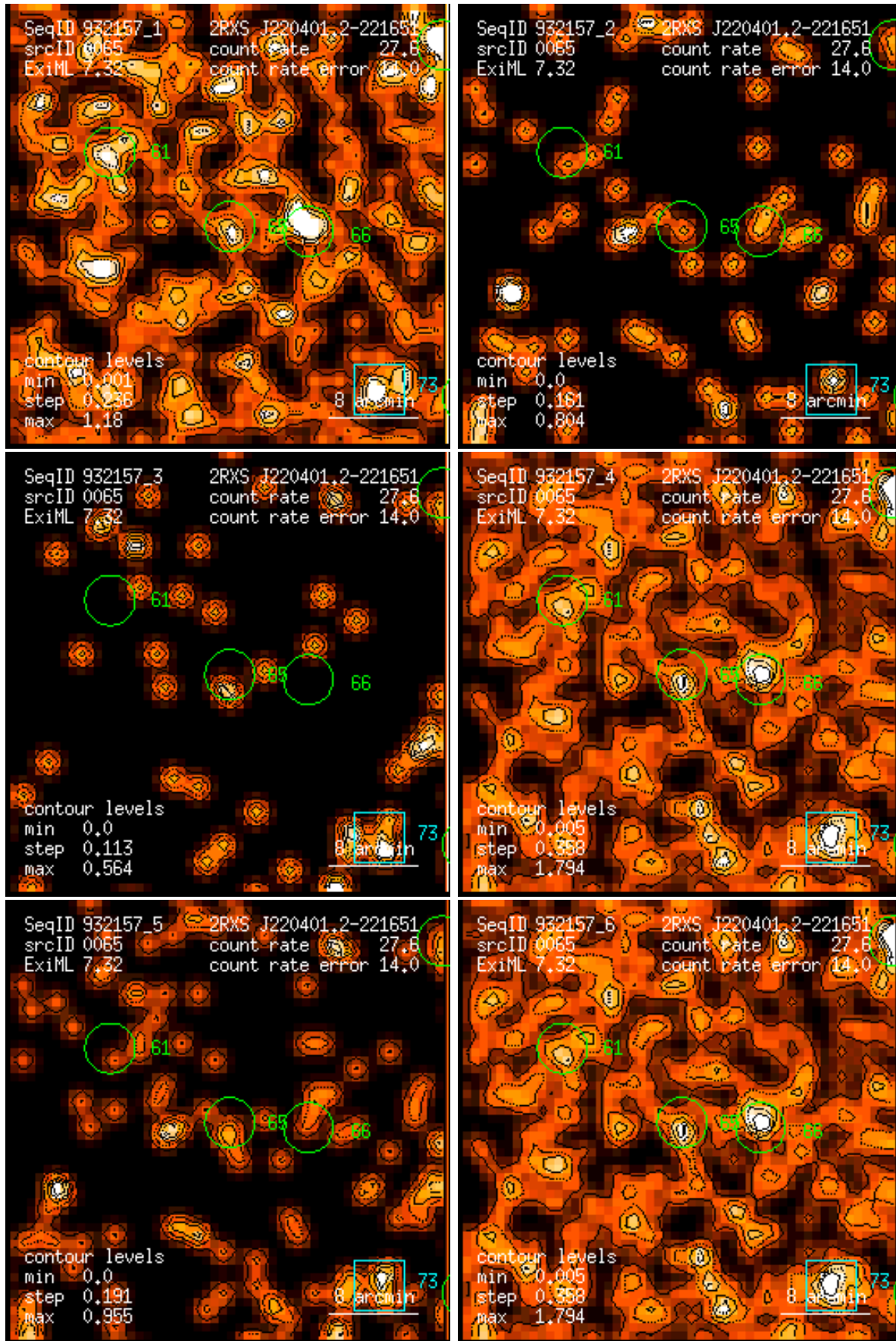
Figure 65: RASS 932157: detection 0065: band rate images, Gaussian filter: (1) PSPC channels 11 – 41, (2) 52 – 90, (3) 91 – 201, (4) 11 – 235, (5) 52 – 201, (6) 11 – 201. Broad band rates in counts/ks. Band rate contour levels in counts/ks/arcmin 2 .
