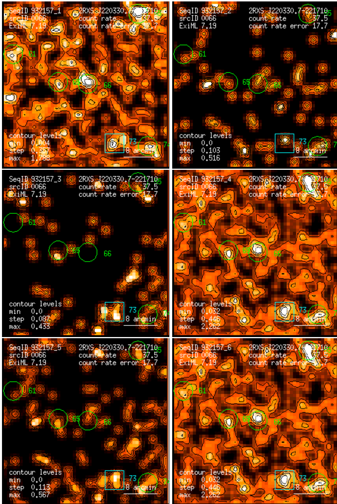
Figure 66: RASS 932157: detection 0066: band rate images, Gaussian filter: (1) PSPC channels 11 – 41, (2) 52 – 90, (3) 91 – 201, (4) 11 – 235, (5) 52 – 201, (6) 11 – 201. Broad band rates in counts/ks. Band rate contour levels in counts/ks/arcmin 2 .
