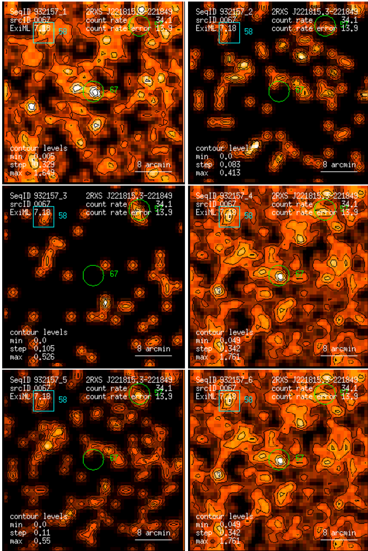
Figure 67: RASS 932157: detection 0067: band rate images, Gaussian filter: (1) PSPC channels 11 – 41, (2) 52 – 90, (3) 91 – 201, (4) 11 – 235, (5) 52 – 201, (6) 11 – 201. Broad band rates in counts/ks. Band rate contour levels in counts/ks/arcmin 2 .
