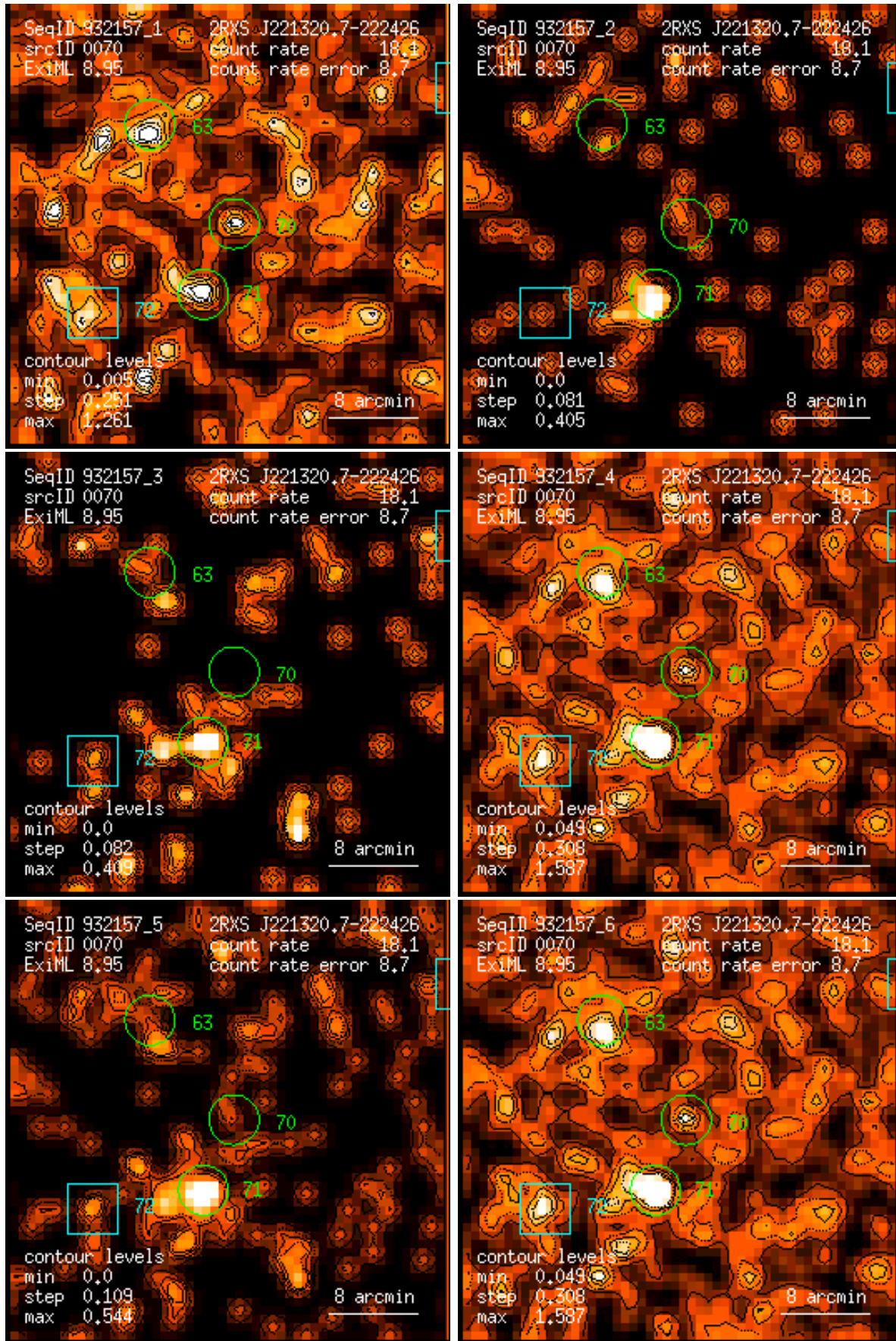
Figure 70: RASS 932157: detection 0070: band rate images, Gaussian filter: (1) PSPC channels 11 – 41, (2) 52 – 90, (3) 91 – 201, (4) 11 – 235, (5) 52 – 201, (6) 11 – 201. Broad band rates in counts/ks. Band rate contour levels in counts/ks/arcmin 2 .
