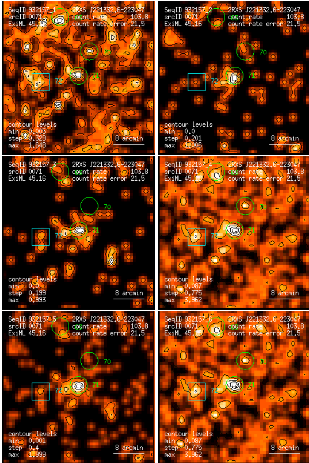
Figure 71: RASS 932157: detection 0071: band rate images, Gaussian filter: (1) PSPC channels 11 – 41, (2) 52 – 90, (3) 91 – 201, (4) 11 – 235, (5) 52 – 201, (6) 11 – 201. Broad band rates in counts/ks. Band rate contour levels in counts/ks/arcmin 2 .
